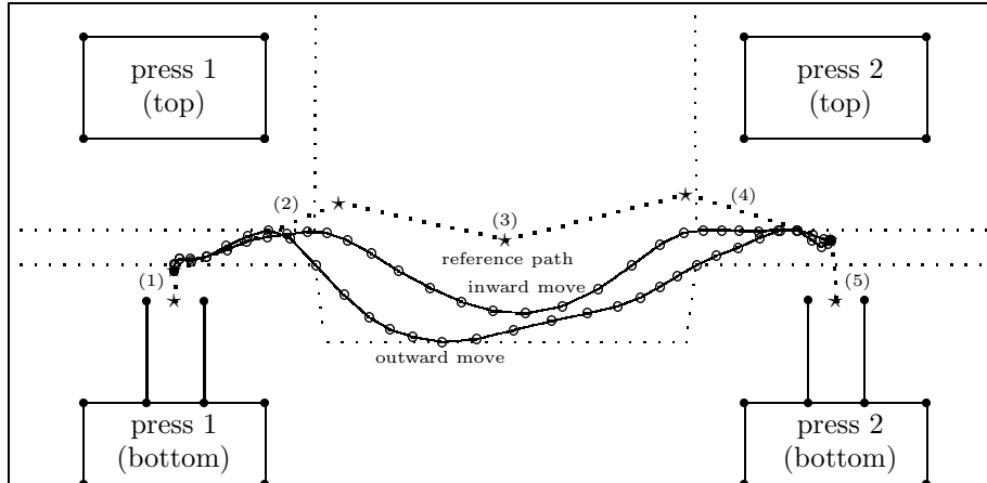
Figure 7: Front view of the press connection workcell (not to scale)
