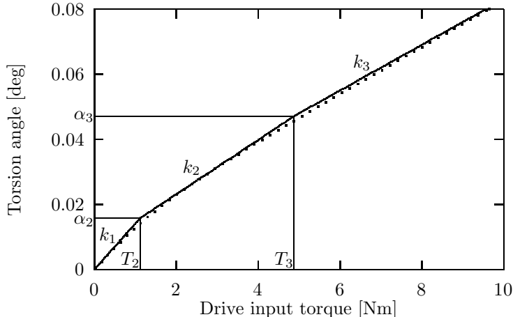
Figure 3: Torsion stiffness of the harmonic drive HDUR-50
