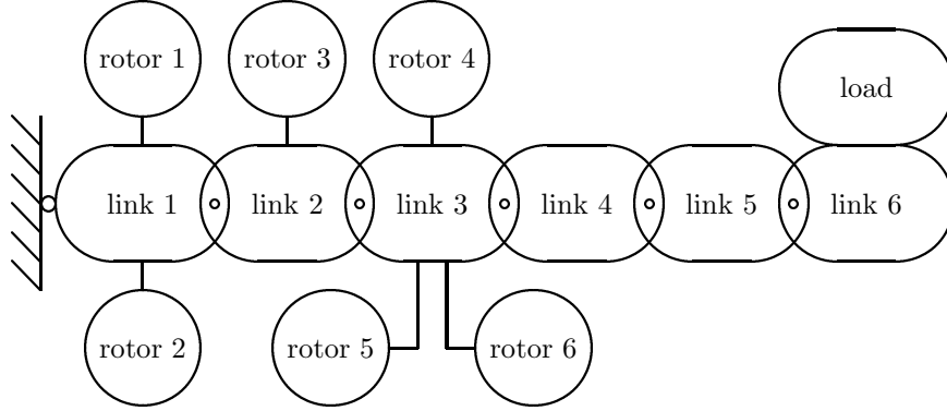
Figure 2: Tree topology of KUKA IR 761 with rotors
