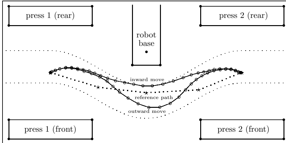
Figure 8: Top view of the press connection workcell (not to scale)
