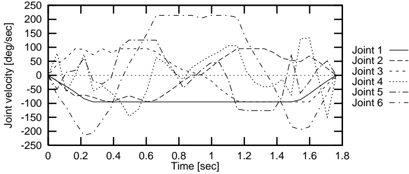
Figure 9: Optimal velocity profiles for outward move
