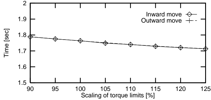
Figure 11: Optimal maneuver time vs. maximal torques
