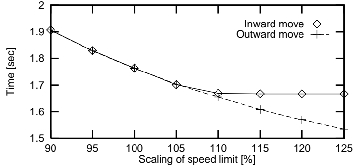
Figure 10: Optimal maneuver time vs. speed limit on first joint
