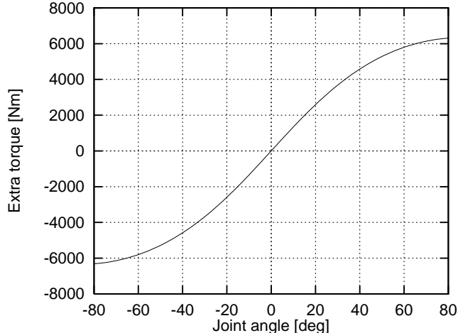
Figure 6: Pneumatic extra torque on the second axis of KUKA IR 761
