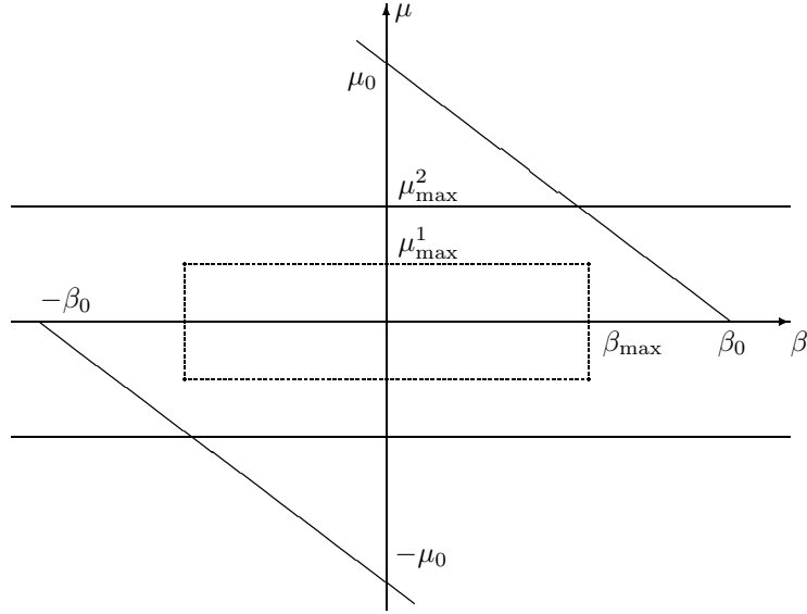
Figure 4: Torque and speed limits for an electric drive
