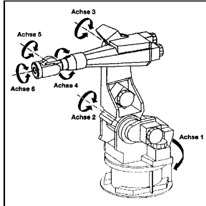
Figure 1: The 6-joint industrial robot KUKA IR 761/125/150.0
