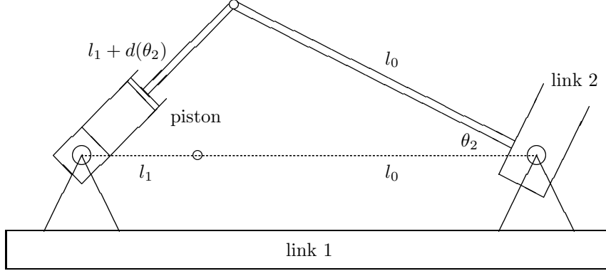
Figure 5: Geometry of pneumatic weight compensation system on KUKA IR 761
