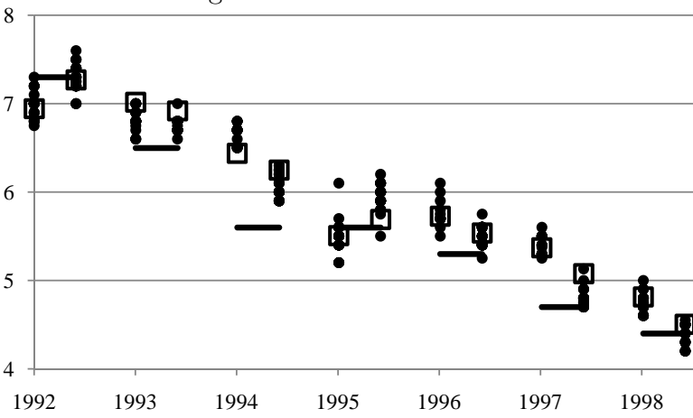
Figure 2: Inflation Forecasts
