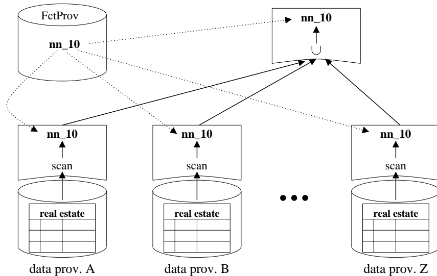
Figure 3.4: Parallel Execution in ObjectGlobe
