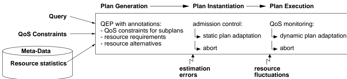
Figure 6.2: The Interaction of Query Processing and QoS Management
