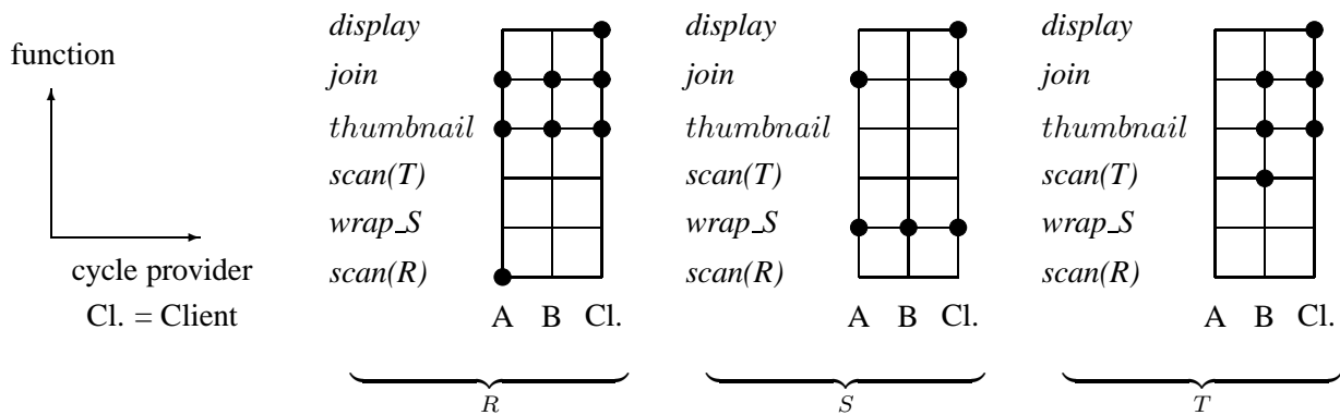
Figure 4.5: Compatibility Matrices for the Example of Section 3.2.2
