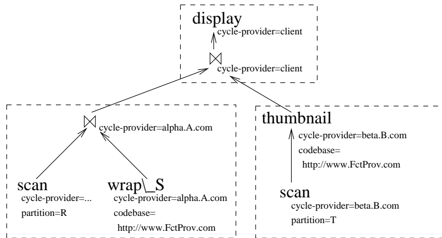
Figure 3.3: Annotated Query Execution Plan
