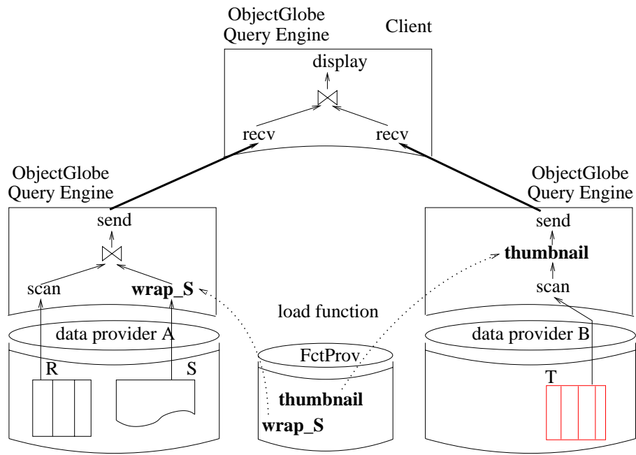
Figure 3.2: Distributed Query Processing with ObjectGlobe
