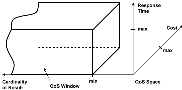
Figure 7.5: The QoS Space and the QoS Window.
