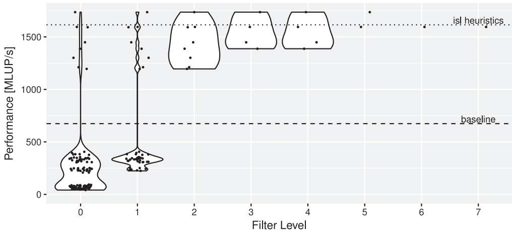
Fig. 6. Performance distribution of all filter levels for Jacobi 2D vc1.
