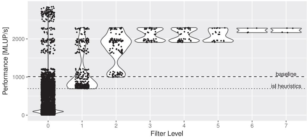
Fig. 7. Performance distribution of all filter levels for RBGS 3D cc1.
