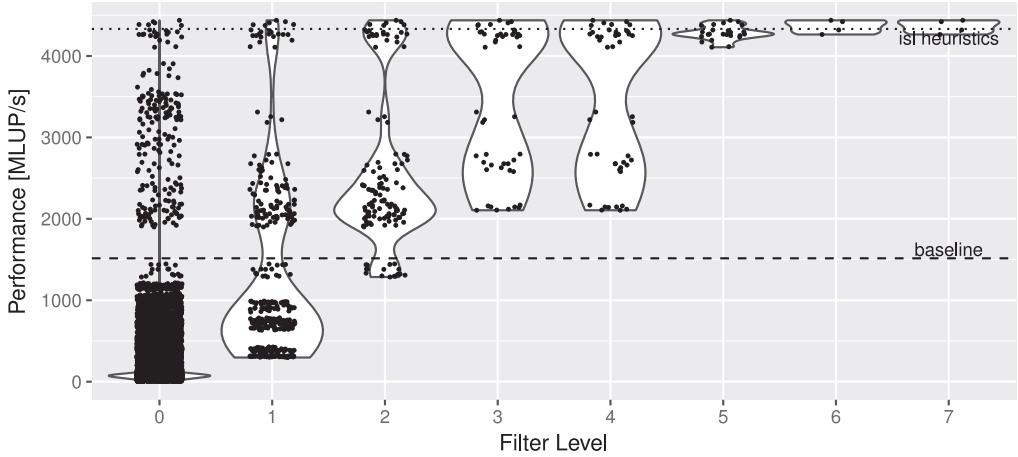
Fig. 5. Performance distribution of all filter levels for Jacobi 3D cc1.
