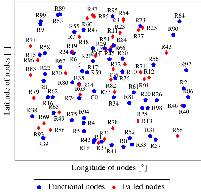
(a) Time 0s: 40 nodes are compromised in the communication network G_C .
