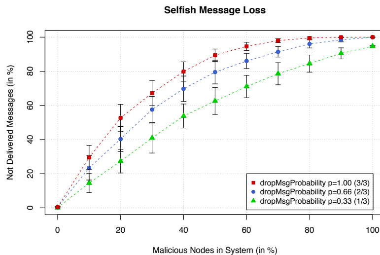
Figure 4.9: Some example graphs are shown for the Scribe [2] system, which have been generated with RCourse. This is the (sorted) node stress distribution (upper graph), the distribution of subscription table entries (middle graph) and message loss due to selfishness-driven message drops (bottom graph).
