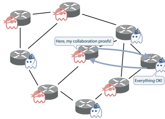
Figure 6.8: In proactive systems, the inspectees decide themselves when to prove correct behaviour in terms of the collaborative protocol. To this end, they transmit on their own – corresponding to an assigned policy – collaboration proofs to an inspector.
