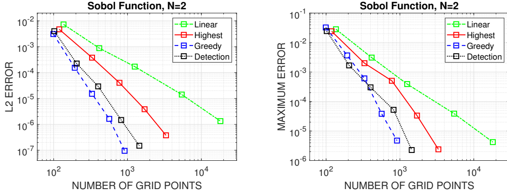
Figure 8: Test problem with f_2^2 . Comparison of the errors \epsilon_2 (left) and \epsilon_\infty (right) for thresholds w_{\max} = 10^{-i} , i = 2, \dots, 6 .
