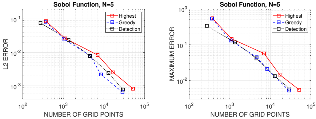
Figure 9: Test problem with f_2^5 . Comparison of the errors \epsilon_2 (left) and \epsilon_\infty (right) for various thresholds w_{\max} \in [10^{-3}, 10^{-1}] .
