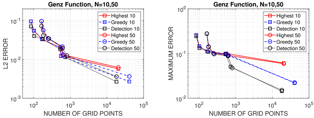
Figure 6: Test problem with f_1^{10,50} . Comparison of the errors \epsilon_2 (left) and \epsilon_\infty (right) for various thresholds w_{\max} \in [3 \cdot 10^{-3}, 10^{-1}] .
