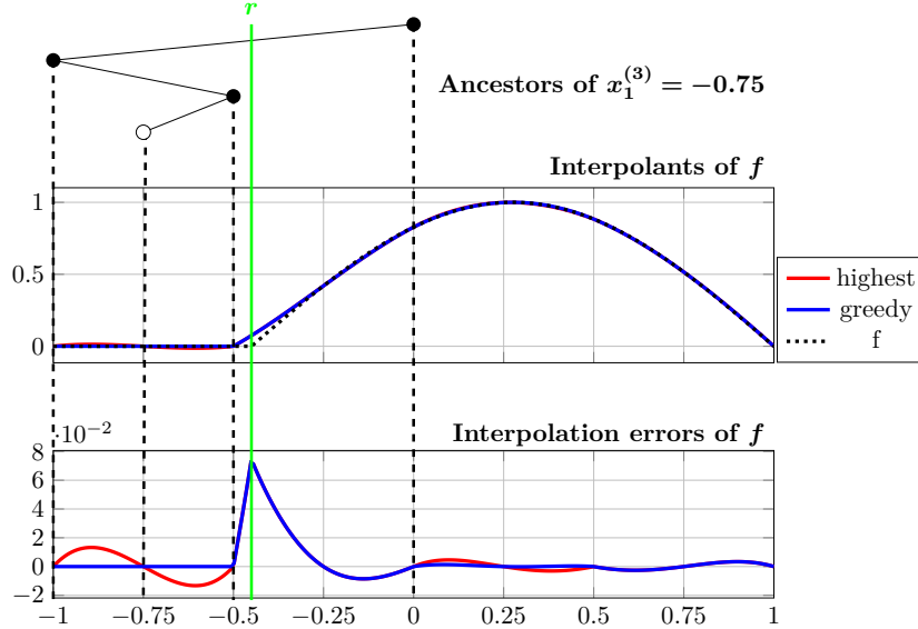
Figure 2: Interpolation across a kink for f defined in (10). The basis function \varphi_{1,3}^{(3)} at knot x_1^{(3)} = -0.75 with highest possible polynomial degree p = 3 uses a function value at x = 0 , which leads to a relatively bad approximation of f(x) \equiv 0 in its support [-1, -0.5] away from the kink at x = -0.45 . The greedy approach described in Section 3.1 restricts the used ancestors and yields a zero error there.
