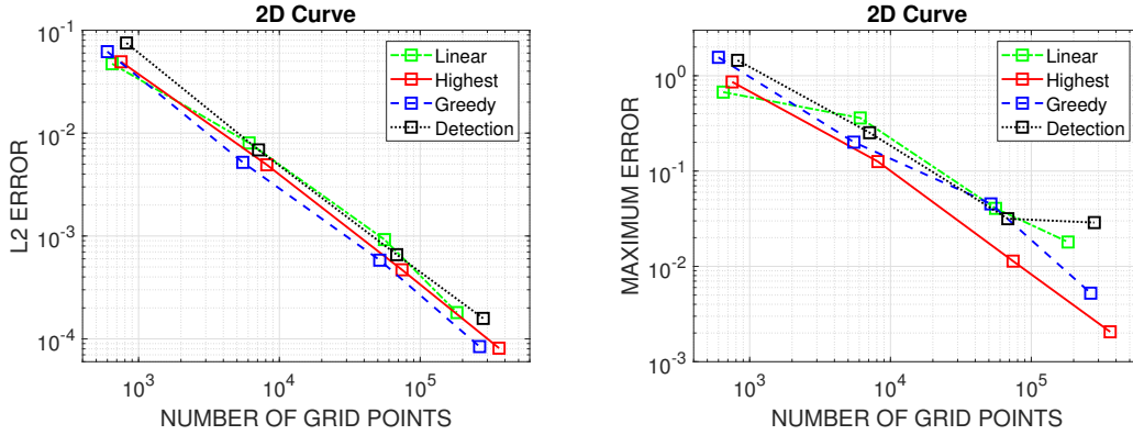
Figure 4: Test problem with f_0 . Comparison of the errors \epsilon_2 (left) and \epsilon_\infty (right) for thresholds w_{\max} = 10^{-i} , i = 1, \dots, 4 .
