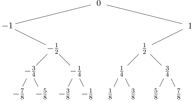
Figure 1: The first 5 levels of the equidistant knot tree on [-1, 1] . For example, the ancestors of knot x = -\frac{5}{8} are S_A(-\frac{5}{8}) = \{-\frac{3}{4}, -\frac{1}{2}, -1, 0\} .
