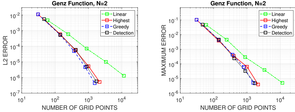
Figure 5: Test problem with f_1^2 . Comparison of the errors \epsilon_2 (left) and \epsilon_\infty (right) for thresholds w_{\max} = 10^{-i} , i = 2, \dots, 6 .
