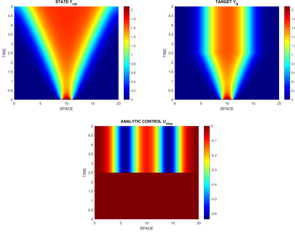
Figure 4: Nucleation process. Y_{nat} for U = 0 (top, left), target function Y_Q (top, right) and analytic control U_{stop} (bottom).
