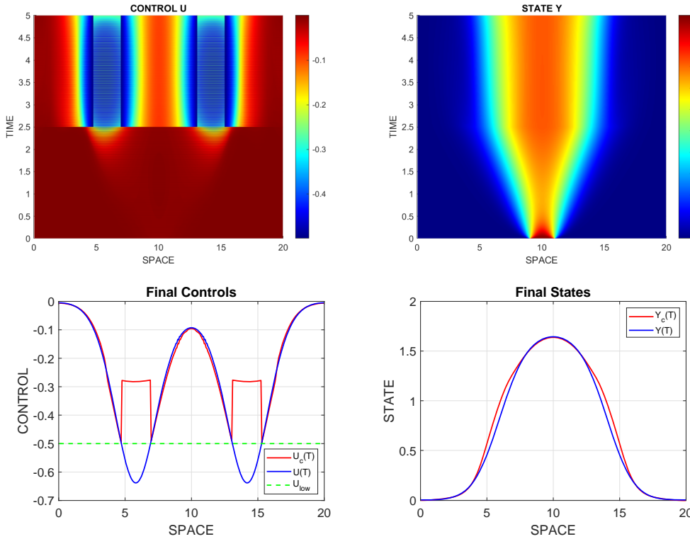
Figure 5: Nucleation process with box constraints for the control. Computed constrained control U_c(t) (top left), state Y_h(t) (top right), constraint and unconstrained controls at final time t = T (bottom left), and corresponding final states (bottom right) approximated by AP4o43p with 50 uniform time steps.
