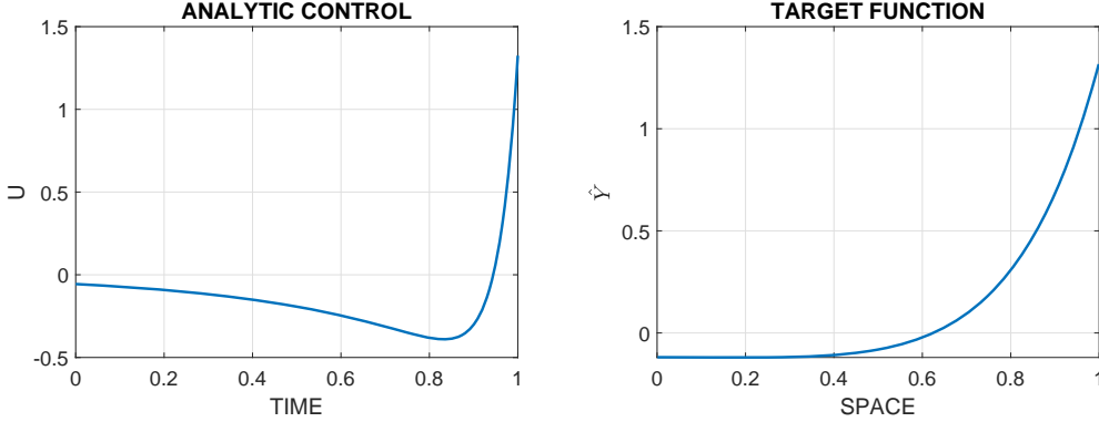
Figure 2: Dirichlet heat problem with m = 500 spatial points. Analytic control u(t) (left) and target function \hat{y} (right).
