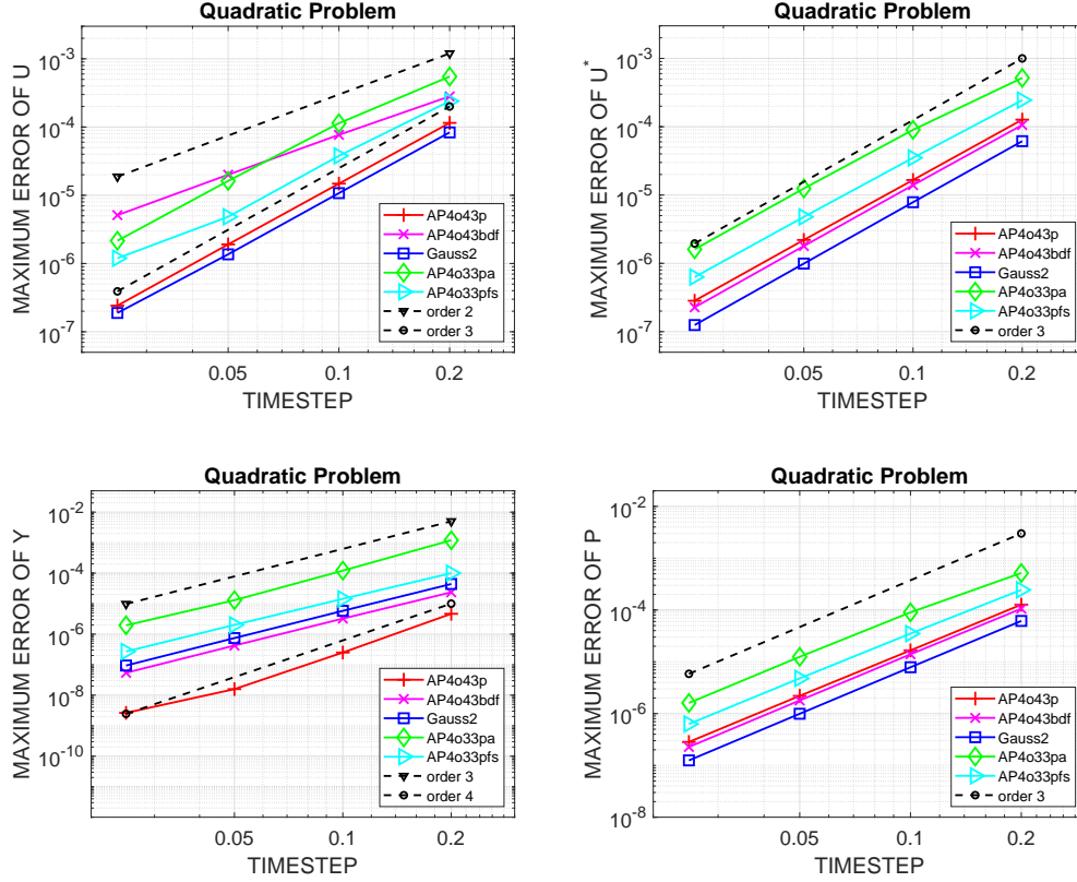
Figure 1: Quadratic Problem. Convergence of the maximal control errors \|U_{ni} - u(t_{ni})\|_\infty (top left), improved control errors \|U_{ni}^* - u(t_{ni})\|_\infty (top right), state errors \|Y_{ni,1} - y_1(t_{ni})\|_\infty (bottom left), and adjoint errors \|P_{ni,1} - p_1(t_{ni})\|_\infty , n = 0, \dots, N , i = 1, \dots, s .
