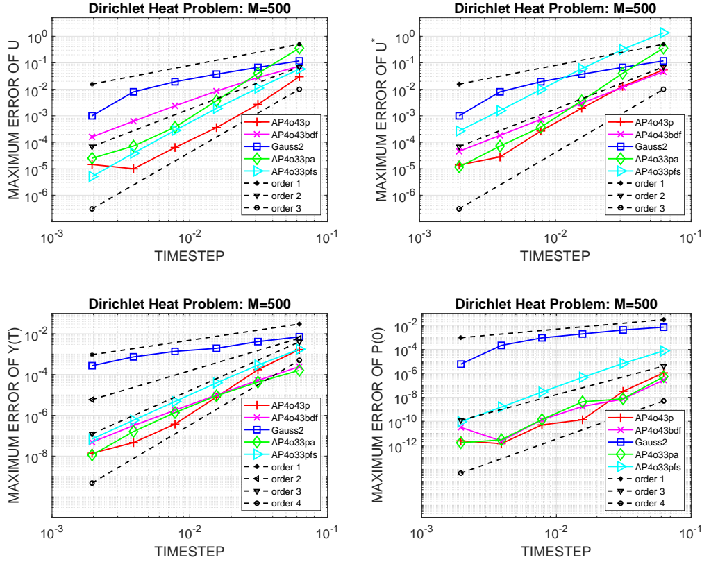
Figure 3: Dirichlet heat problem with m = 500 spatial points. Convergence of the maximal control errors \|U_{ni} - u(t_{ni})\|_\infty (top left), improved control errors \|U_{ni}^* - u(t_{ni})\|_\infty (top right), state errors \|y(T) - y_h(T)\|_\infty (bottom left), and adjoint errors \|p(0) - p_h(0)\|_\infty (bottom right).
