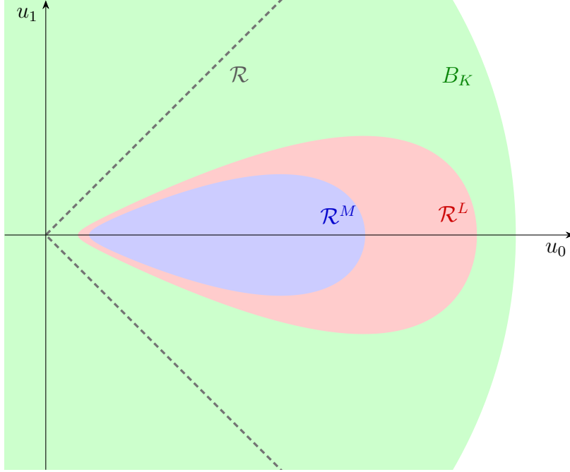
FIGURE 1. The sets used in the proof of Lemma 4.4. For this figure, we consider the M_1 case in slab geometry: V = [-1, 1] , \mathbf{m}(v) = (1, v) . In this case, the realizable set is given by \mathcal{R} = \{(u_0, u_1) : |u_1| < u_0\} , and we used M = 1 , L = 1.3 , and K = 8 .
