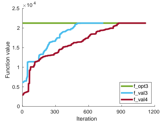
Figure 5: Comparison of the third optimization for non robust feasible GasLib-40 with and without warm start
