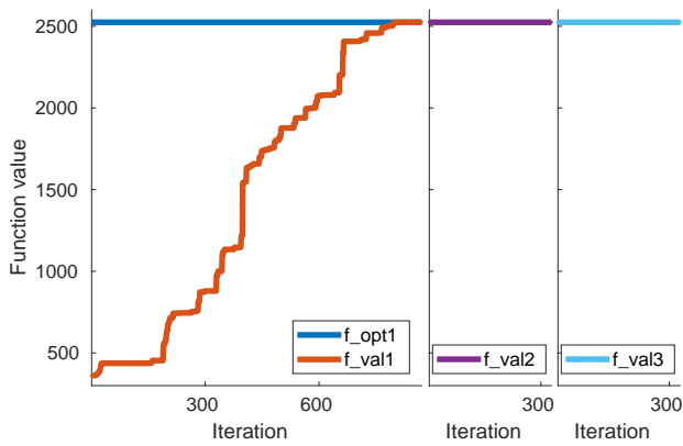
Figure 6: Optimization history of CASM for the non robust feasible GasLib-134 instance
