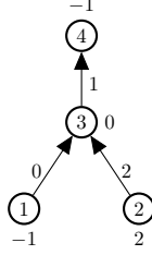
Figure 5: Network problem (node labels b , arc labels u ), in which shrinking of (1, 3) leads to a missed IIS.
