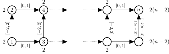
Figure 4: Network problem (node labels b , arc labels [\ell, u] ) with an exponential number of minimal INCs.
