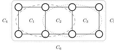
Figure 10: Graph with \alpha = 6 elementary cycles.
