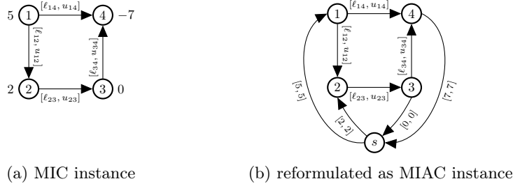
Figure 7: Example for the transformation from a network instance where node and arc violations are allowed to a circulation instance where only arc violations are permitted; node labels (on the left side) b , arc labels [\ell, u] .
