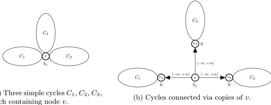
Figure 9: Transformation from simple cycles sharing a single node to elementary cycles; node labels b , arc labels [\ell, u] .
