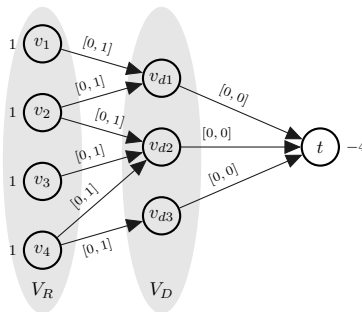
Figure 2: Sketch of the construction for the reduction from set cover to IAC, with ground set R = \{1, 2, 3, 4\} and subset collection D = \{\{1, 2\}, \{2, 3, 4\}, \{4\}\} ; node labels b , arc labels [\ell, u] .
