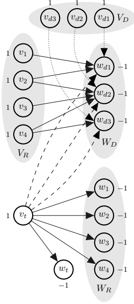
Figure 8: Sketch of the construction for the reduction from set cover to IAC for assignment problems, where R is the ground set and D is the collection of subsets of the set cover instance. All arc bounds are [\ell, u] = [0, 1] .
