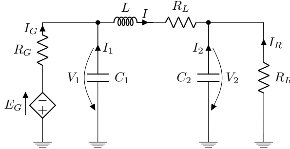
Figure 1: Basic DC power network example
