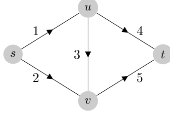
Figure 2: A diamond shaped network, with source s and sink t and arc labels 1 to 5.
