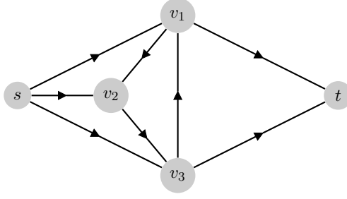
Figure 5: A graph for which dicycle inequalities (11) define facets of \mathcal{P}^{\text{AS}\pm} .
