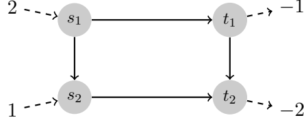
Figure 3: The graph shows that Theorem 15 does not hold for |\mathcal{V}_+|, |\mathcal{V}_-| \geq 2 : Suppose that b_{s_2}, b_{t_2} \neq 0 and b_{s_2} < -b_{t_2} , then the flow on at least one of the arcs (s_1, s_2) and (t_1, t_2) has to be positive. Nevertheless, if b_{t_1} \neq 0 , they need not be used in \mathcal{P}^{\text{AS}\pm} , i.e., \mathcal{P}^{\text{AS}\pm} \not\subseteq \mathcal{P}^{\text{AF}} .
