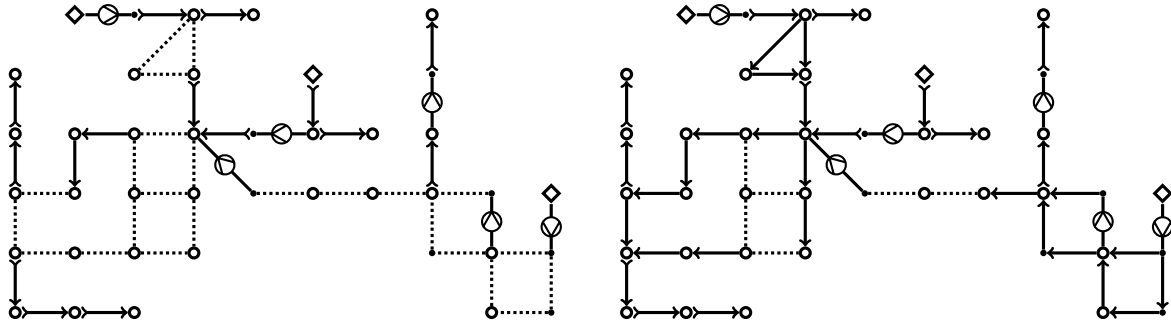
Figure 6: The presolved network GasLib-40 corresponding to variants NFD (left) and FLC+AC (right). The scenario has 3 sources (diamonds) and 29 sinks (circles). Pipes with fixed flow are depicted by \rightsquigarrow , fixed flow directions are shown by \rightarrow , and the remaining pipes (with unfixed flows/directions) are dashed.
