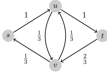
Figure 4: The graph \mathcal{D}(z^+, z^-) associated with a vertex of \mathcal{P}_{\text{LP}}^{\text{AS}\pm} applied to the network of Figure 2.
