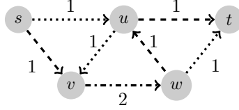
Figure 1: An s - t -flow which can be decomposed into two paths (indicated by dashed/dotted arcs) each with flow value 1, but is not acyclic.
