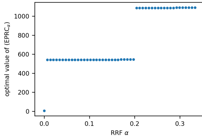
FIGURE 4. Trade-off between robustness and cost, i.e., optimal value of robust counterpart ( \text{EPRC}_{\alpha} ) as a function of the size of \alpha \bar{U}_j, j \in J , for instance comp07-2idx with RRF \rho_{\text{MIP}} = 0.3333 .
