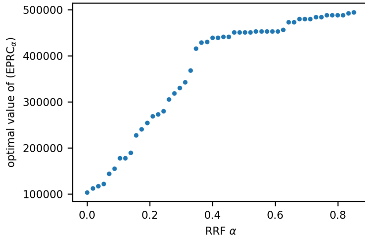
FIGURE 5. Trade-off between robustness and cost, i.e., optimal value of robust counterpart ( \text{EPRC}_\alpha ) as a function of size of \alpha \bar{U}_j, j \in J , for instance drayage-100-23 with \text{RRF } \rho_{\text{MIP}} = 0.8509 .
