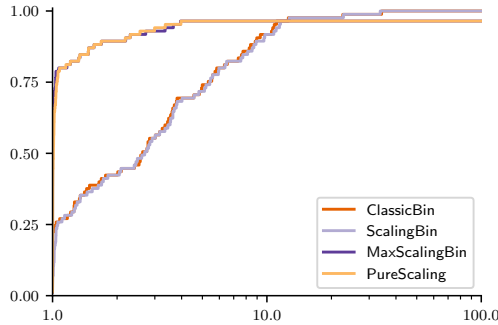
FIGURE 2. Log-scaled performance profiles of runtimes for instances with RRF zero
