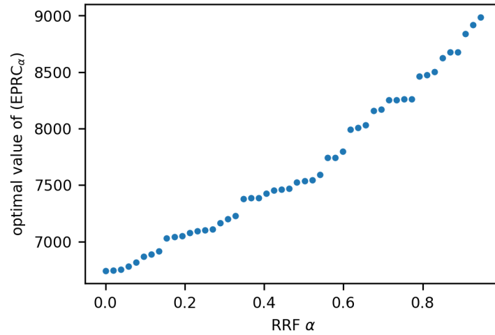
FIGURE 3. Trade-off between robustness and cost, i.e., optimal value of robust counterpart ( \text{EPRC}_{\alpha} ) as a function of the size of \alpha \bar{U}_j, j \in J , for instance binkar10_1 with RRF \rho_{\text{MIP}} = 0.9459 .
