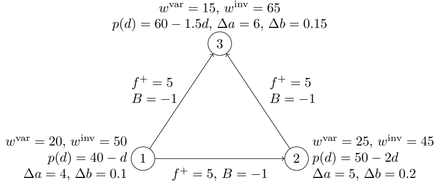
FIGURE 2. 3-node network with the technical, economic, and uncertainty data used in the computational study
