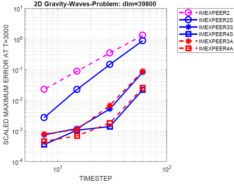
Figure 4: Nonlinear Two-Dimensional Gravity Waves: Scaled maximum errors at T = 3000 taken over all system components vs. time step sizes. Comparison of IMEX-Peer methods.
