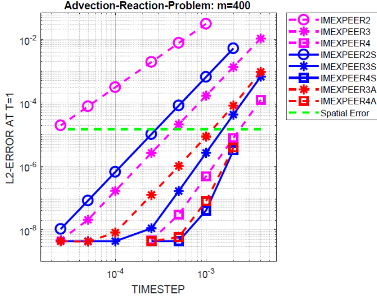
Figure 3: Advection-Reaction-Problem: l_2 -errors at T = 1 of the total concentration vs. time step sizes, m = 400 . Comparison of IMEX-Peer methods. Results that correspond to failures or unstable numerical solutions are not shown.
