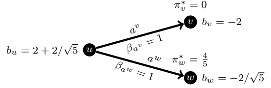
Figure 6: Binary decision gadget with exactly two possibilities for u 's potential: \pi_u^1 = \pi_u^2 = 1 or \{\pi_u^1, \pi_u^2\} = \{0, 4\}
