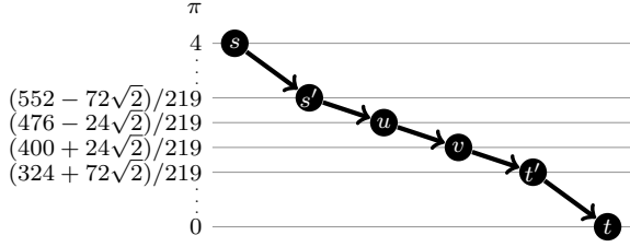
Figure 2: Node potentials of a maximum feasible stationary gas s - t -flow of value \sqrt{(76 - 48\sqrt{2})/219} \approx 0.193 on the path network described in Example 7
