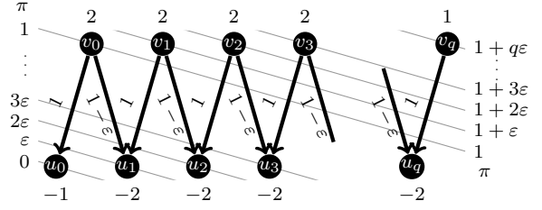
Figure 3: Node potentials \pi \in \mathbb{R}^V inducing a stationary gas b/2 -flow in the path network of Example 9; the numbers at arcs indicate the \beta_a -values, the numbers at nodes b_u -values.
