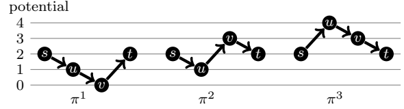
Figure 1: Node potentials of 3-stage gas s - t -flow with value 2 - \sqrt{2} on the path network described in Example 6
