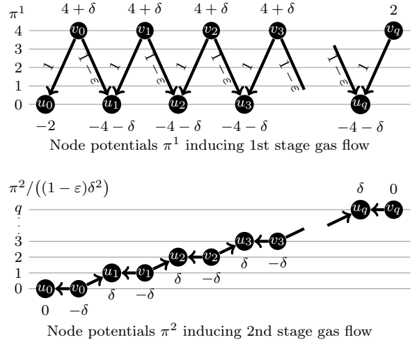
Figure 4: Node potentials \pi^1 and \pi^2 inducing an instationary 2-stage gas b -flow in the network of Example 9; here \delta := 2/\sqrt{1 - \varepsilon} - 2 \in \theta(\varepsilon) for \varepsilon \rightarrow 0 .
