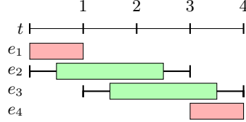
Fig. 8. Example for an unbounded power of preemption.
