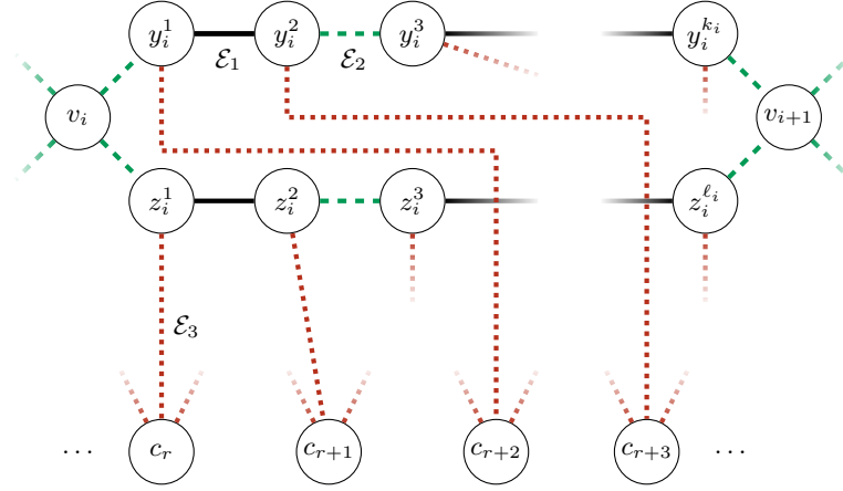
Fig. 3. Schematic representation of the gadget for variable x_i , which appears negated in clause C_r and positive in clause C_{r+2} among others.
