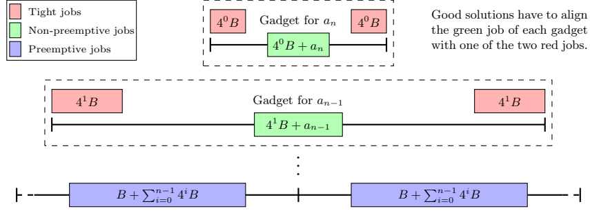
Fig. 9. Instance created from a PARTITION instance a_1, \dots, a_n, B . The number inside the blocks are the processing times of the jobs.
