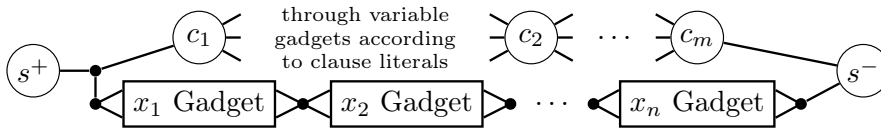
Fig. 2. High-level view of the construction for Theorem 3.
