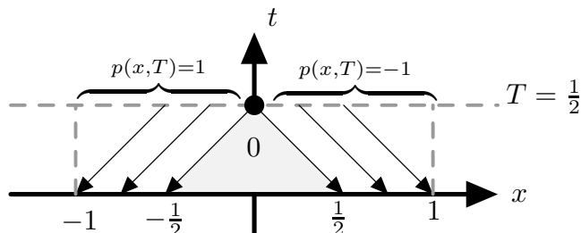
FIG. 1. Construction of the adjoint using the method of characteristics in space-time domain. Note that the adjoint has a constant value in the gray area due to the discontinuity of the state at time T .
