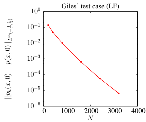
FIG. 5. Convergence of the discrete adjoint computed using the Lax-Friedrich method.
