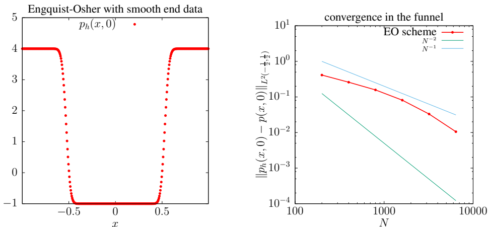
FIG. 7. Discrete adjoint at t = 0 (left) and convergence of the discrete adjoint to its continuous counterpart in the shock funnel (right).
