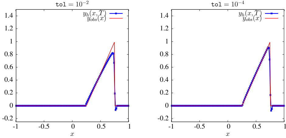
FIG. 8. The state variable y_h(x, T) obtained from optimization algorithm with \text{tol} = 10^{-2} and \text{tol} = 10^{-4} .
