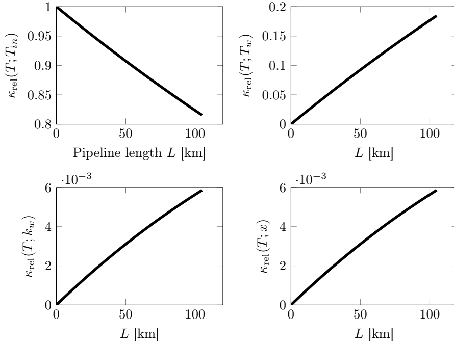
Figure 6: The individual relative condition numbers \kappa_{\text{rel}}(T; T_{\text{in}}) , \kappa_{\text{rel}}(T; T_w) , \kappa_{\text{rel}}(T; k_w) , and \kappa_{\text{rel}}(T; x) in (65) considered as a function of the pipeline length L = x - x_0 for concrete values (66).
