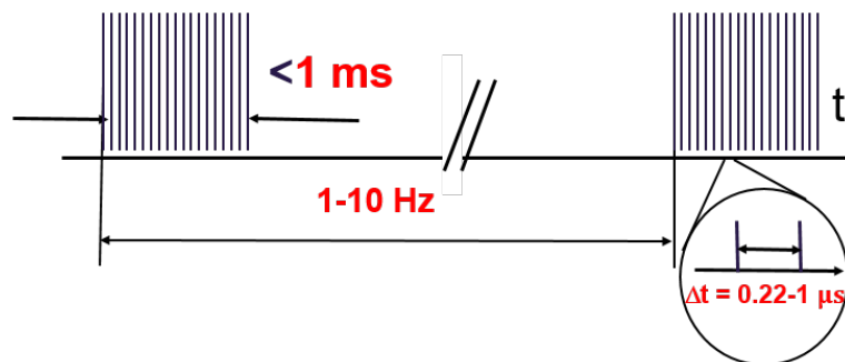
Figure 1. Electron bunch train structure at PITZ.
