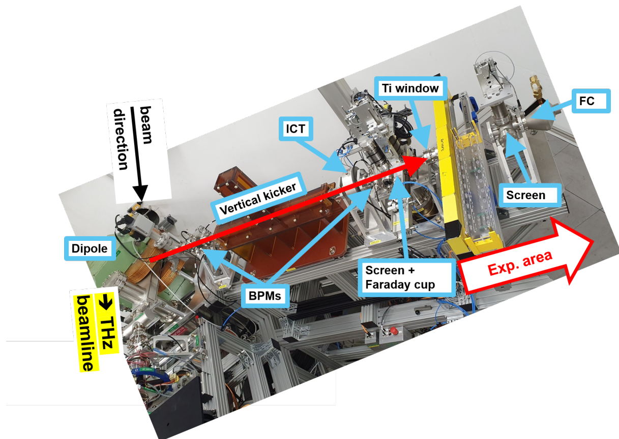
Figure 2. Startup beamline for FLASHlab@PITZ.
