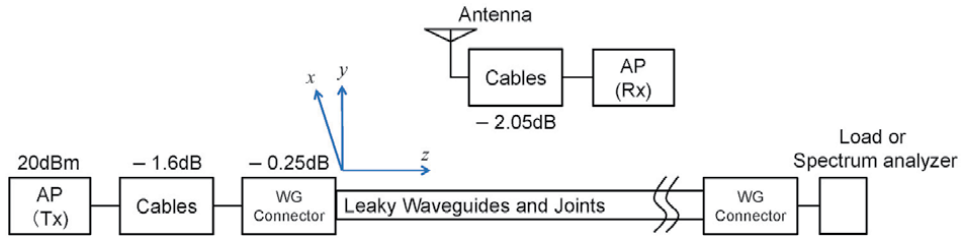
Figure 20. Experimental configuration.
