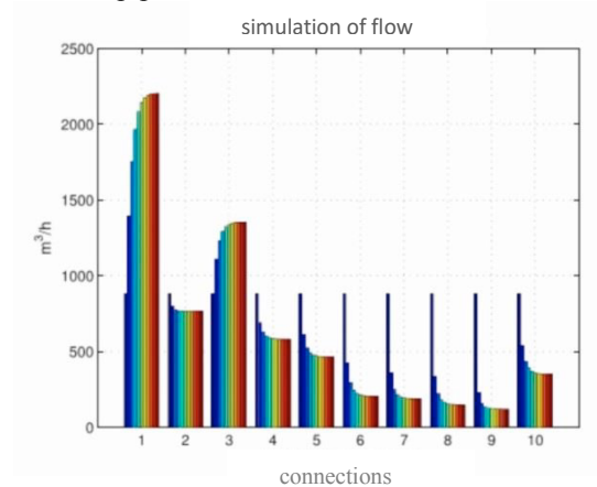
Fig. 10: Simulation with number of branches method: flow in pipe connections 1-10
