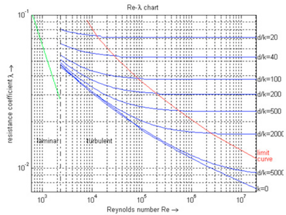
Fig. 3. Re - \lambda chart
