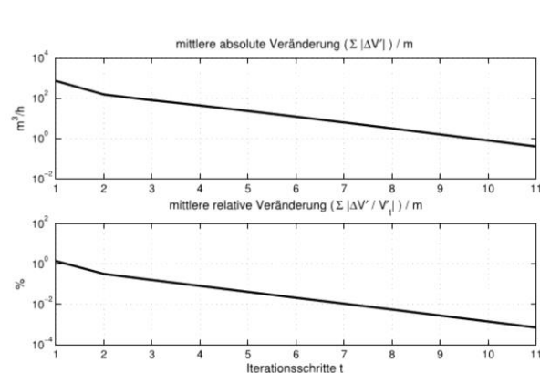
Fig. 7: Simulation with random method: flow change and number of iterations
