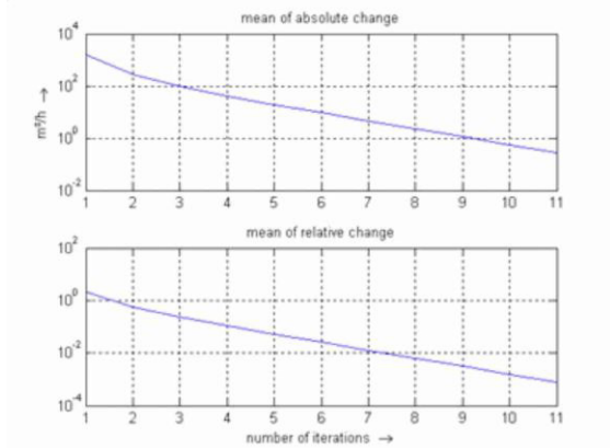
Fig. 6: Simulation with maximum method: flow in pipe connections 1-10
