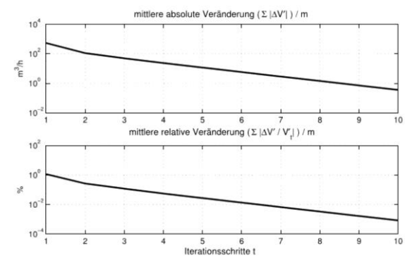
Fig. 9: Simulation with number of branches method: flow change and number of iterations
