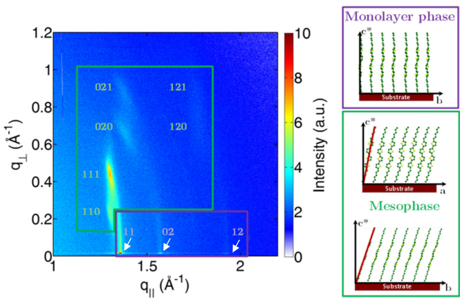
Fig. 4 2D-GIXD pattern of a DH4T film measured at 110^\circ\text{C}
