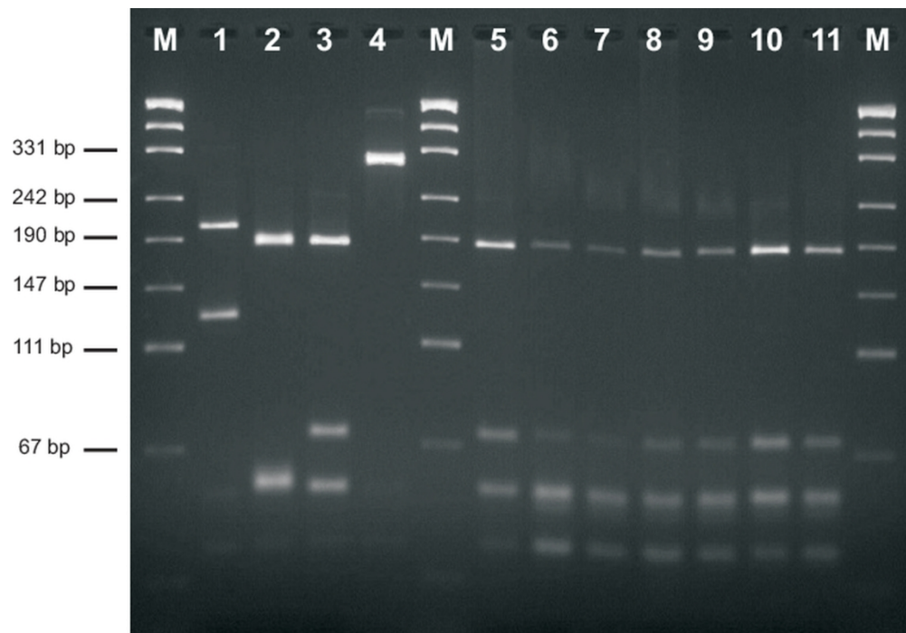
Figure 2. ITS1-PCR-RFLP of ITS1 with HaeIII of reference strains and representative clinical samples of the Armenian studied cases. M, pUC19 DNA size marker; 1-3, WHO-reference strains: 1, L. major MHOM/SU/1973/5ASKH; 2, L. tropica MHOM/SU/1974/SAF-K27; 3, L. infantum MHOM/ES/1993/PM1; 4, ITS1 undigested clinical sample; 5, Arm8; 6, Arm3; 7, Arm5; 8, Arm6; 9, Arm7; 10, Arm9; 11, Arm10
