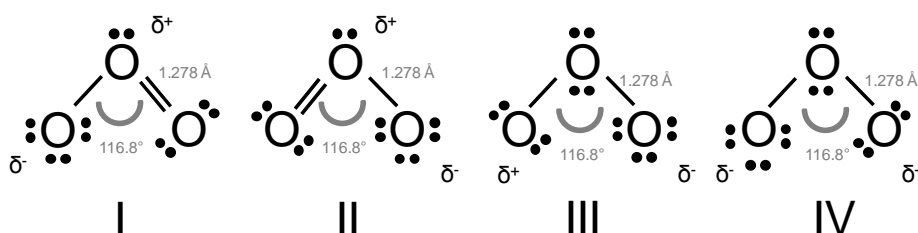
Figure 2.5: Resonance structures of ozone molecules (Trambarulo et al. , 1953).
