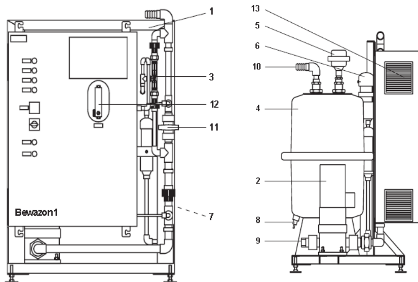
1. Rack; 2. Booster pump; 3. Injector; 4. Tank; 5. Vent valve; 6. Annihilation of residual ozone; 7. Water reservoir; 8. Drain valve; 9. Water entrance; 10. Water outlet; 11. Bypass valve; 12. Gas flow meter; 13. Air filter
