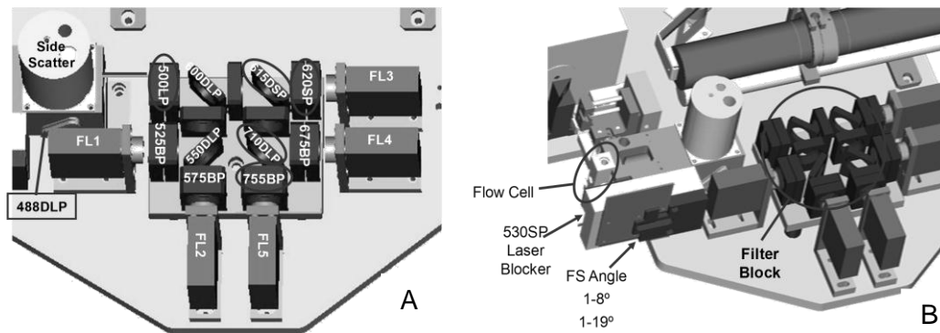
Figure 2.14: Optical system of the Cytomics FC 500. A) Design-layout of the flow cytometer. B) Optical layout of the flow cytometer (Beckman Coulter).
