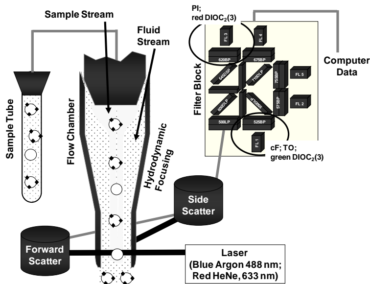
Figure 3.2: Principle of Cytomics FC500.
