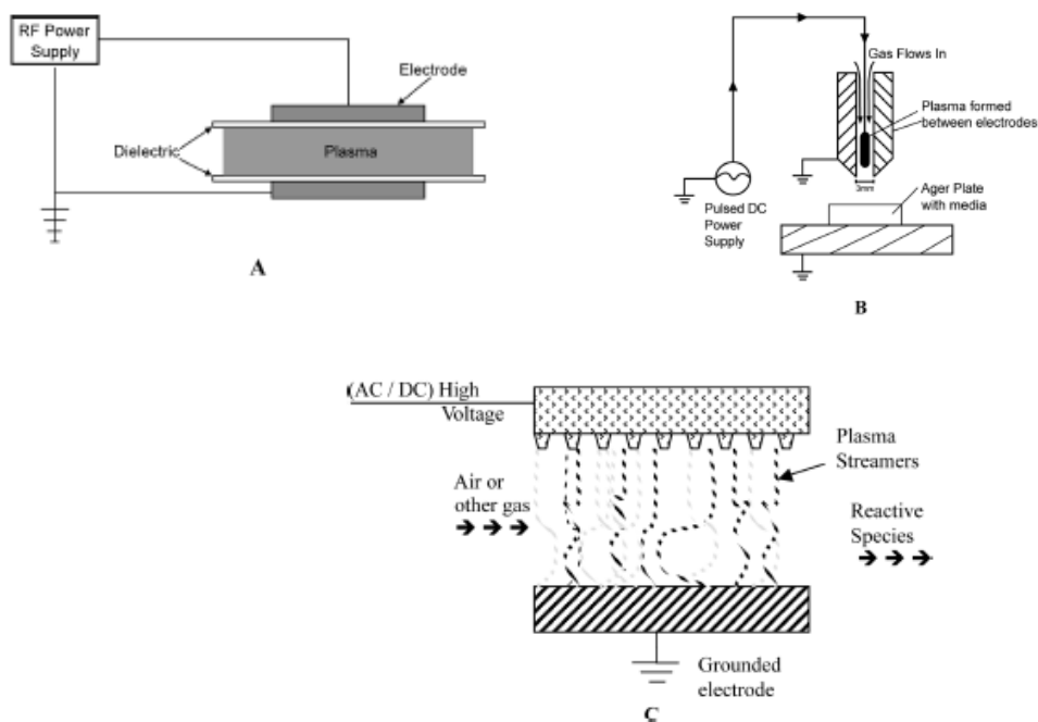
Figure 2.10: Atmospheric pressure plasma generation systems: A) dielectric barrier discharge, B) plasma jet, C) corona discharge (Keener, 2008).
