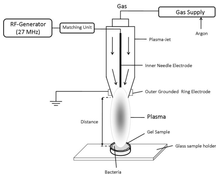
Figure 3.7: Experimental set-up of the used atmospheric pressure plasma jet.
