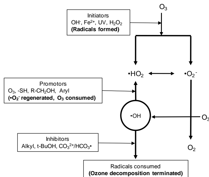
Figure 2.6: Ozone decomposition reactions (modified after Khadre et al. , 2001).
