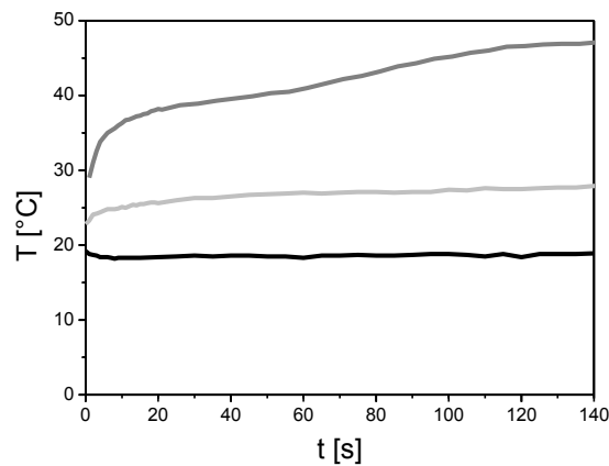
Figure 4.9: Development of sample surface temperature due to plasma treatment at different power levels. Black line: 10 W; light grey line: 20 W, and grey line: 40 W.
