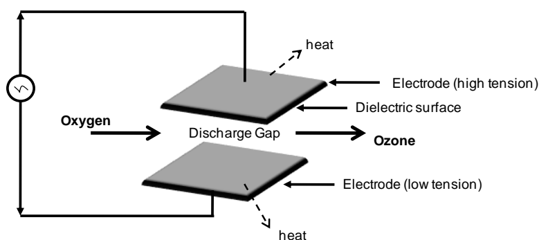
Figure 2.8: Ozone generation by the electrical discharge method (modified after Kim et al. (1999) and Karaca & Velioglu (2007)).
