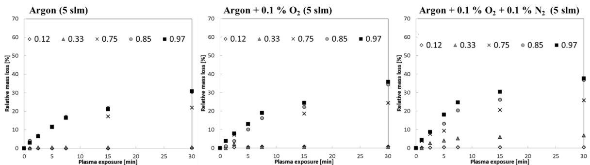
A3. 4: Time dependent mass loss of liquid model systems with varying a_w -values exposed to direct CAPP treatment under variation of the working gas (Bußler, unpublished data).
