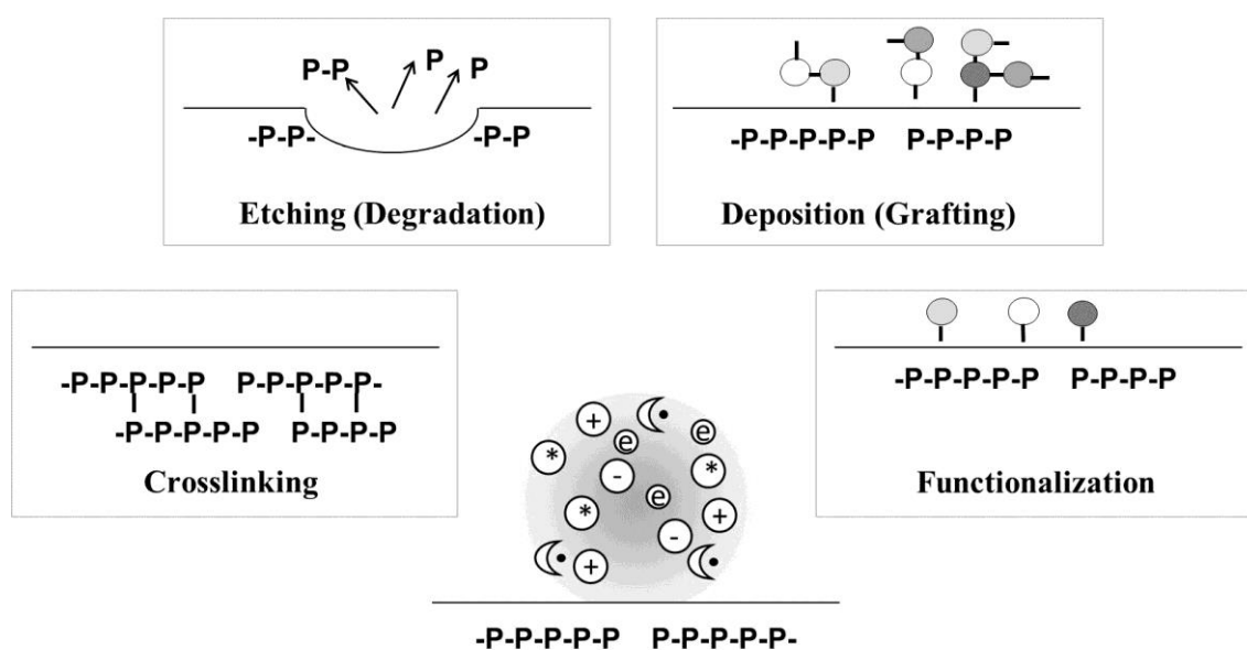
Figure 8: Surface modifying processes that may take place during plasma treatment; adapted from Bazaka et al. [72].
