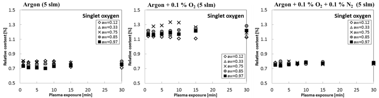
A3. 2: Relative singlet oxygen content of the plasma afterglow during exposure to solid model systems with varying a_w -values under variation of the working gas measured via optical emission spectroscopy (Bußler, unpublished data).
