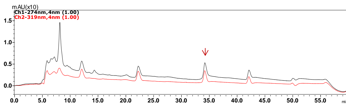
A1. 8: Exemplary RP-HPLC chromatogram of the separation of chlorogenic acid after a 10 min exposure to PPA detected at 274 (black) and 319 nm (red).
