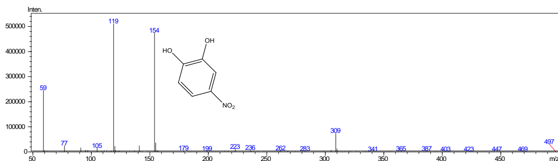
RP C (Retention time = 31.083 min)
