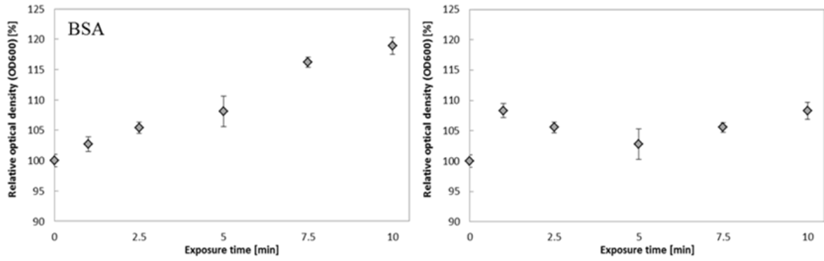
A2. 1: Plasma-induced impact on relative optical density of the model protein solutions BSA (Bovine serum albumin) and \beta -LG (Beta-lactoglobulin) at \lambda = 600 nm (Bußler, unpublished data).
