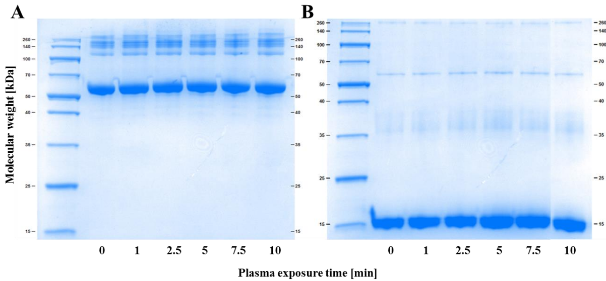
A2. 2: Electrophoretic separation of BSA (A, Bovine serum albumin) and \beta -LG (B, Beta-lactoglobulin) following exposure to direct CAPP treatment for up to 10 min.
