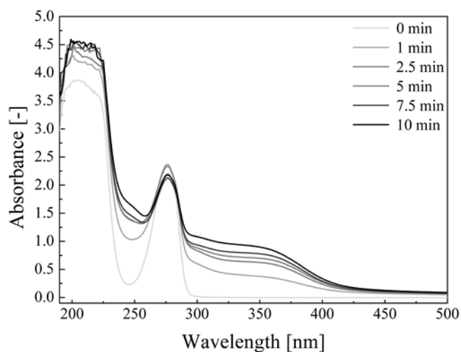
Figure 4: Plasma-induced changes in UV/Vis spectra in pyrocatechol solution (1 mM) dependent on plasma exposure time [min].
