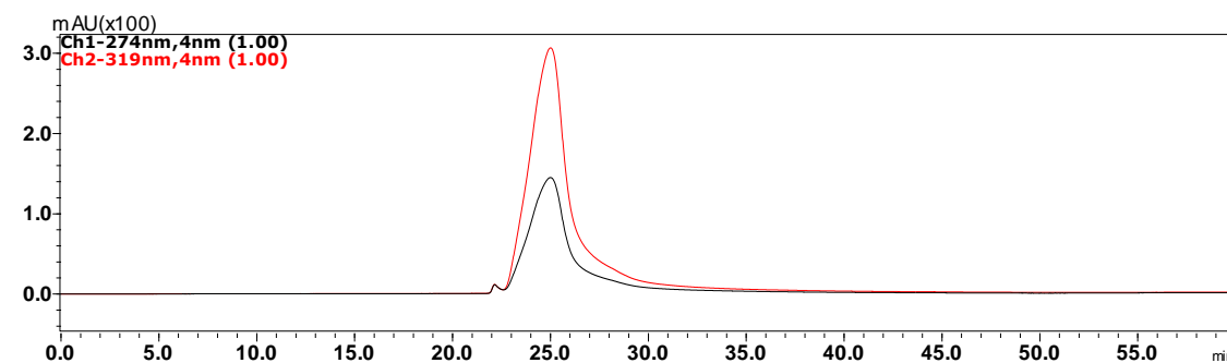
A1. 3: Exemplary RP-HPLC chromatogram of the separation of caffeic acid after a 10 min exposure to PPA detected at 274 (black) and 319 nm (red) and the plasma-induced adduct was also at the same retention time.
