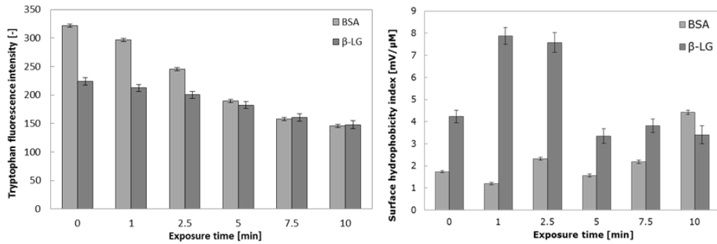
A2. 4: Plasma-induced impact on tryptophan fluorescence intensity (pH 7.0, \lambda_{ex} = 290 nm, \lambda_{em} = 334/348 nm – left) and on surface hydrophobicity (pH 7.0, \lambda_{ex} = 390 nm, \lambda_{em} = 470 nm - right) of \beta -LG and BSA solutions (Bußler, unpublished data).
