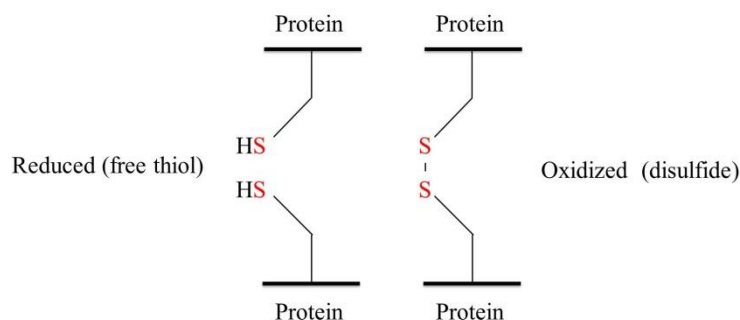
Figure 10: Disulfide (sulfur-sulfur) linkages between two cysteine residues.
