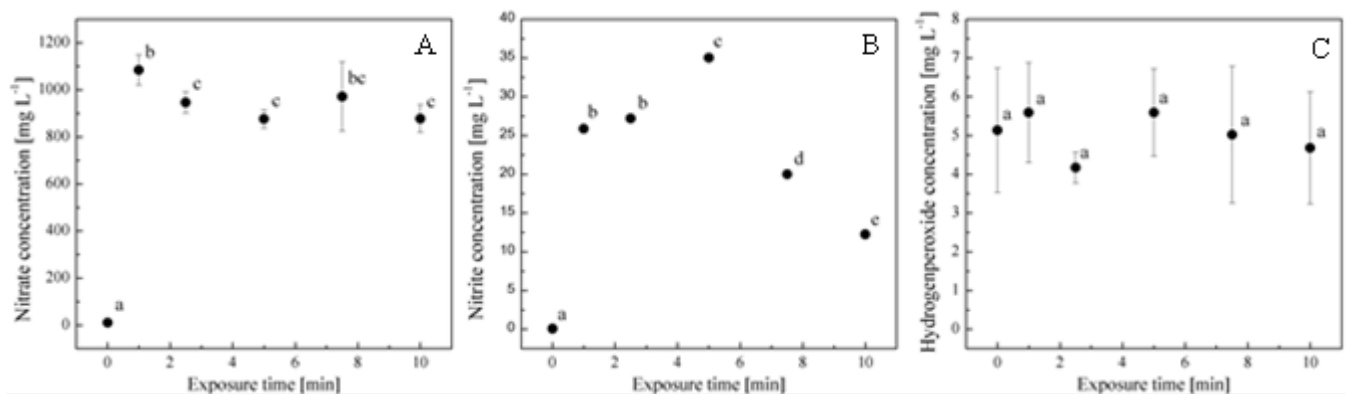
Figure 2: Concentrations of accumulated nitrate (left), nitrite (center) and hydrogenperoxide (right) in pure water depending on plasma exposure time [min]. The results are presented as the mean of six replicates ( n = 6 ) as experimental data. Different small letters (a-e) indicate significantly different values ( p < 0.05 , Tukey's test) for each sample.
