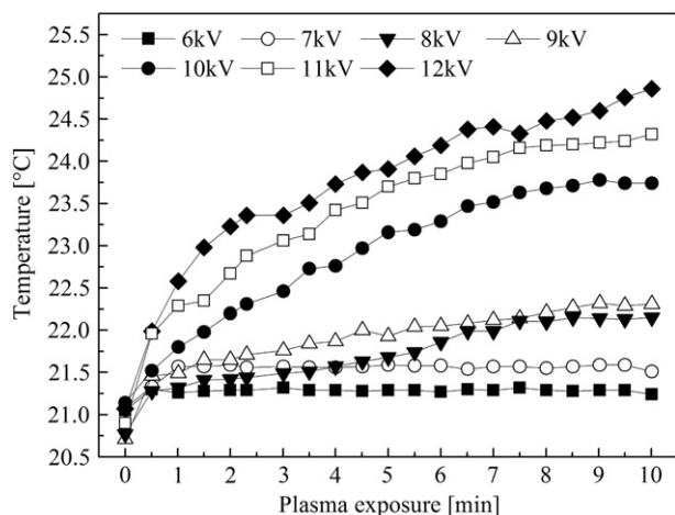
Fig. 3. Temperature in the reaction chamber during plasma treatment in air, varying the applied voltages from 6 to 12 kV pp (3.0 kHz).
