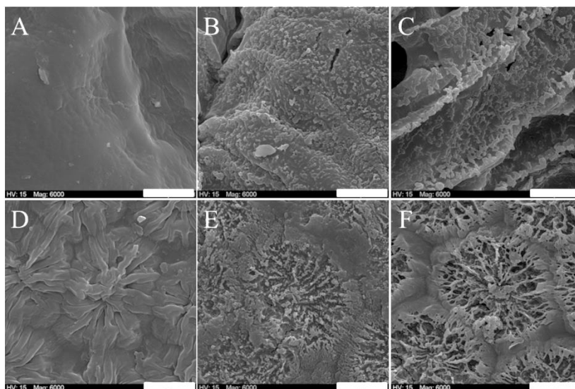
Figure 17: Scanning electron micrographs of morphological outer surface of hulled peas (A-C) and pea testa (D-F) prior to (A and D) and following plasma treatment for 5 min (B and E) and 15 min (C and F), respectively. Scale bars 5 \mu\text{m} , adapted from Bußler et al. [152].
