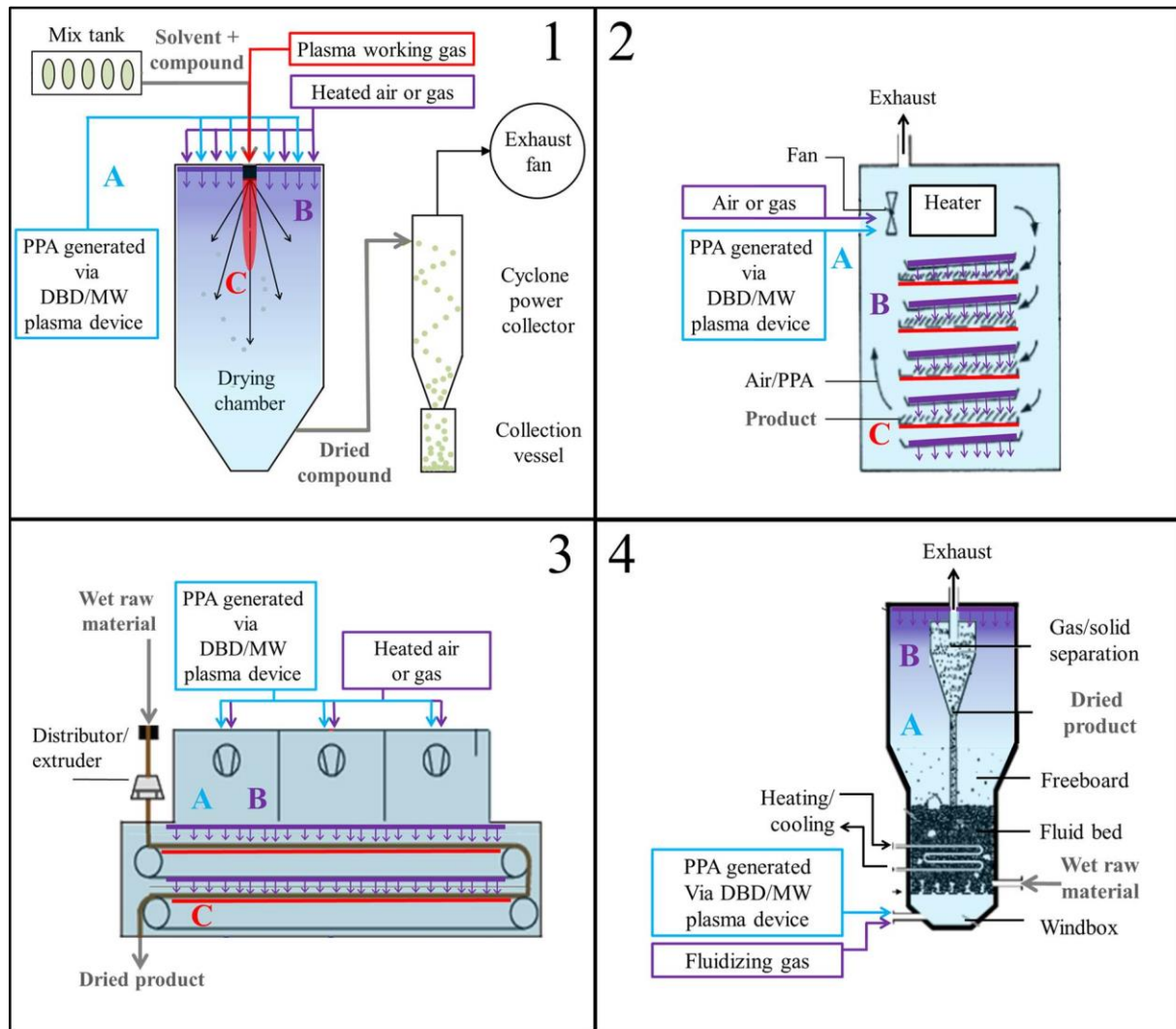
Figure 27: Prospective plasma-drying set-ups realizable by combinations of spray (1), tray (2), belt (3) and fluid bed (4) dryers coupled with plasma-jet, DBD or MW driven plasma devices for the indirect (A), semi-direct (B) and direct (C) CAPP application during drying of liquid and particulate raw materials, intermediates and products.
