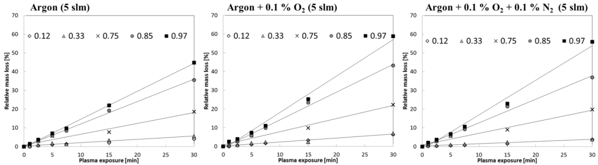
Figure 24: Time dependent mass loss of solid model systems with varying a_w -values exposed to direct CAPP treatment (plasma jet kINPen©) under variation of the working gas (Bußler, unpublished data).
