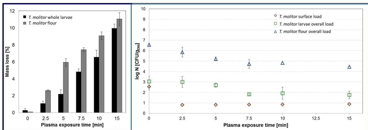
Figure 19: Mass loss of Tenebrio larvae and flour detected following CAPP treatment for up to 15 min (left) and impact of CAPP treatment for up to 15 min on total viable count (TVC) on surface and of whole Tenebrio larvae and on TVC of Tenebrio flour corrected by the respective final dry matter contents (Bußler, unpublished data ).
