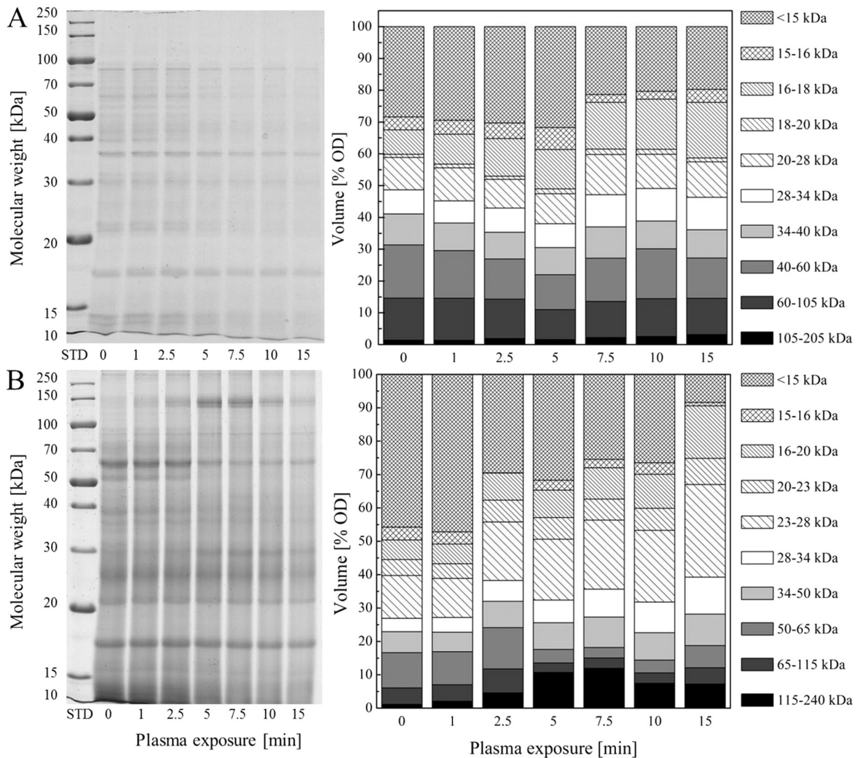
Fig. 5. Electrophoretic separation (left) and relative composition (OD = Optical Density) of soluble protein fractions (right) from Tenebrio flour depending on the CAPP exposure time following extraction at pH 4 (A) and 10 (B), n = 3 .
