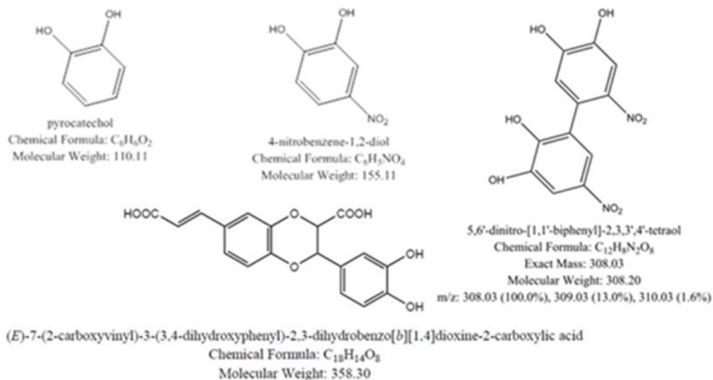
Figure 7: Proposed products of pyrocatechol under conditions of the PPA-mediated reaction
