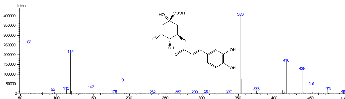
A1. 7: The most prominent m/z value of the untreated chlorogenic acid sample was 353 (Retention time = 22.217 min).
