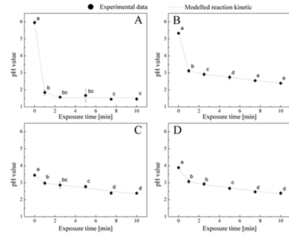
Figure 1: Change of pH in pure water (A), pyrocatechol (B), chlorogenic (C) and caffeic acid (D) solutions (10 mM) depending on plasma exposure time [min]. The results are presented as the mean of six replicates ( n = 6 ) as experimental data. Different small letters (a-e) indicate significantly different values ( p < 0.05 , Tukey's test) for each sample. The dotted lines represent the reaction kinetic obtained from the applied biphasic model.
