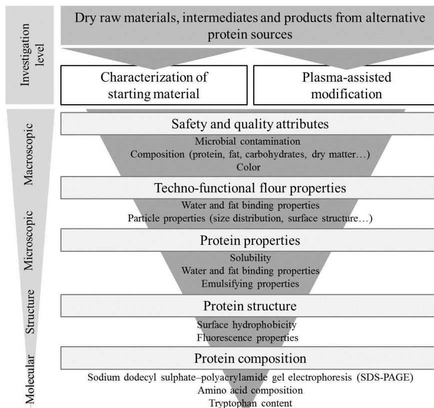
Figure 18: Schematic depiction of the top-down approach in the utilization of analytical methods providing insights into possible underlying plasma-induced mechanisms in protein-rich flours from macroscopic to molecular level.
