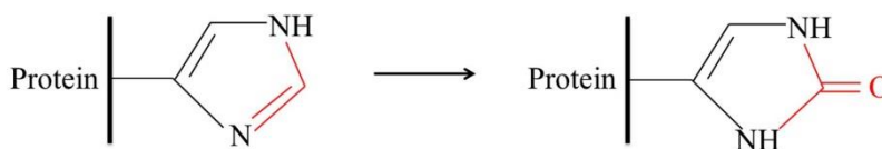
Figure 12: Carbonylation, an irreversible formation of free carbonyl groups, in amino acids.
