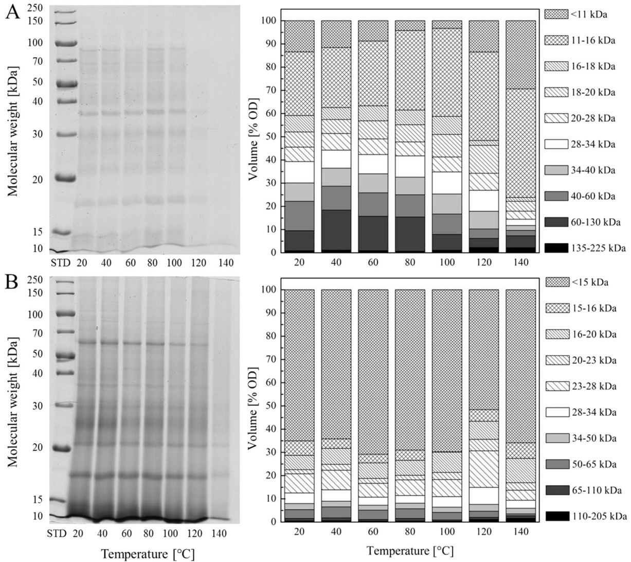
Fig. 4. Electrophoretic separation (left) and relative composition (OD = Optical Density) of soluble protein fractions (right) from Tenebrio flour depending on the treatment temperature following extraction at pH 4 (A) and 10 (B), n = 3 .
