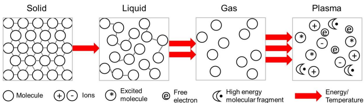
Figure 2: The four fundamental states of matter.
