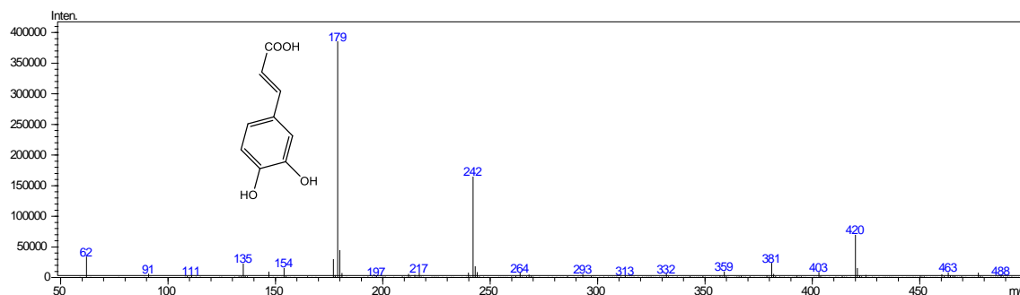
A1. 4: The prominent m/z values of the untreated caffeic acid sample were 179 and 242 (Retention time = 25.40 min).
