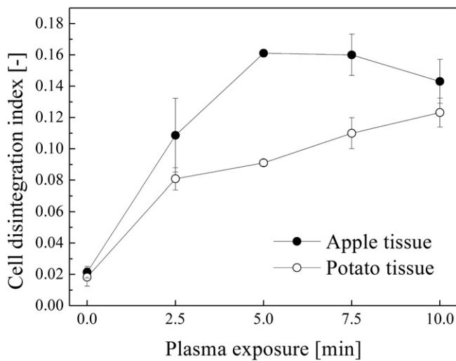
Fig. 3. Impact of PPA treatment on cell disintegration index of fresh cut tissue from apple and potato tuber.
