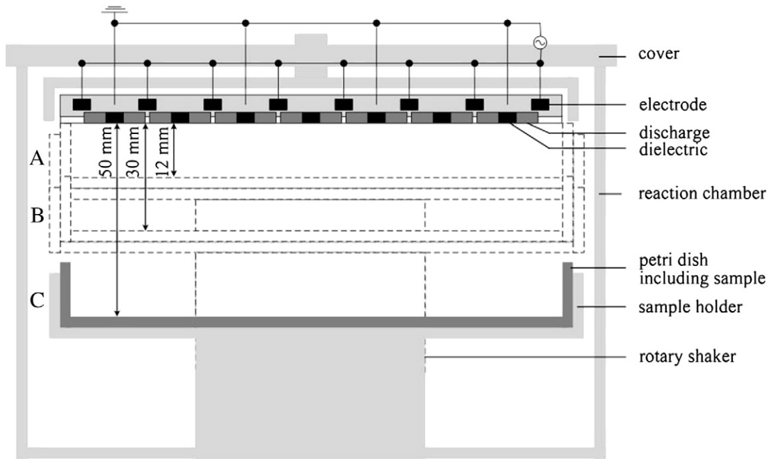
Fig. 1. Experimental set-up of the cold atmospheric pressure surface dielectric barrier discharge plasma device for the treatment of pea seeds (A), sprouts (B) and seedlings (C).
