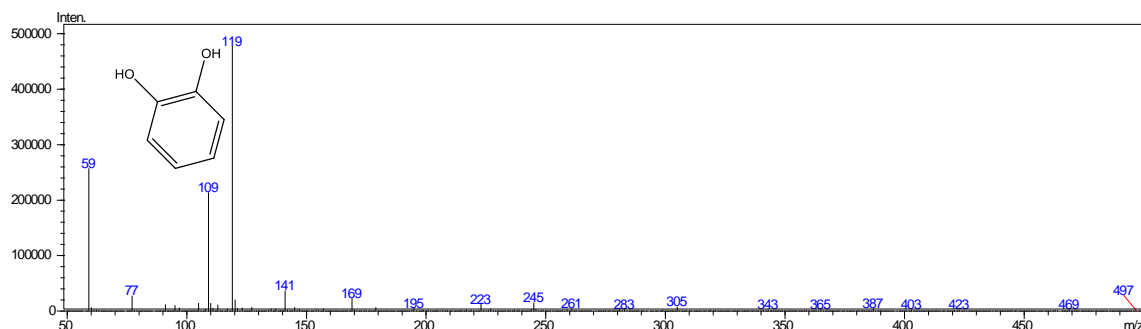
A = Catechol (Retention time = 14.433 min)
