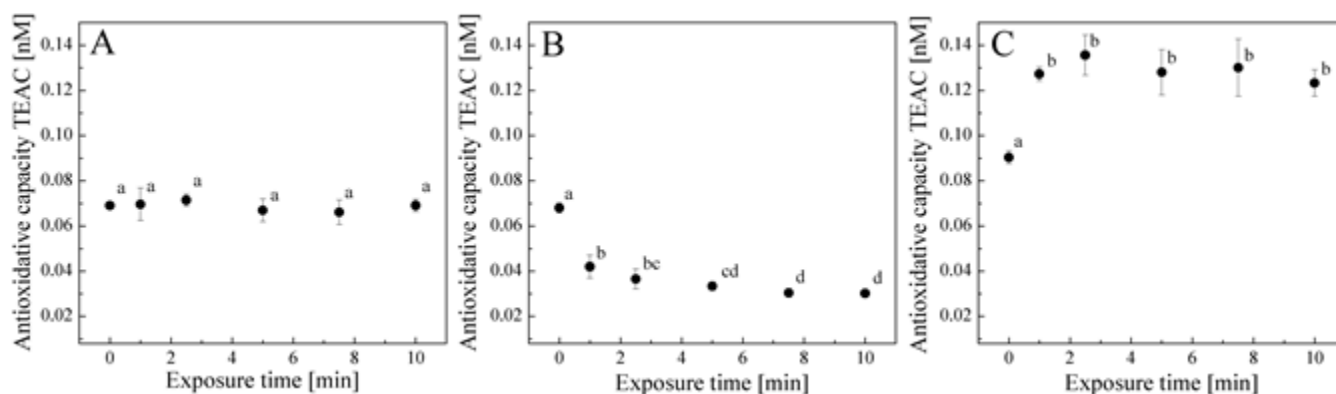
Figure 3: Change of the antioxidative capacity as measured by the TEAC assay in pyrocatechol (A, 1 mM), chlorogenic (B, 0.1 mM) and caffeic (C, 0.1 mM) acidic solutions depending on plasma exposure time [min]. The results are presented as the mean of six replicates ( n = 6 ). Different small letters (a-d) indicate significantly different values ( p < 0.05 , Tukey's test) for each sample.
