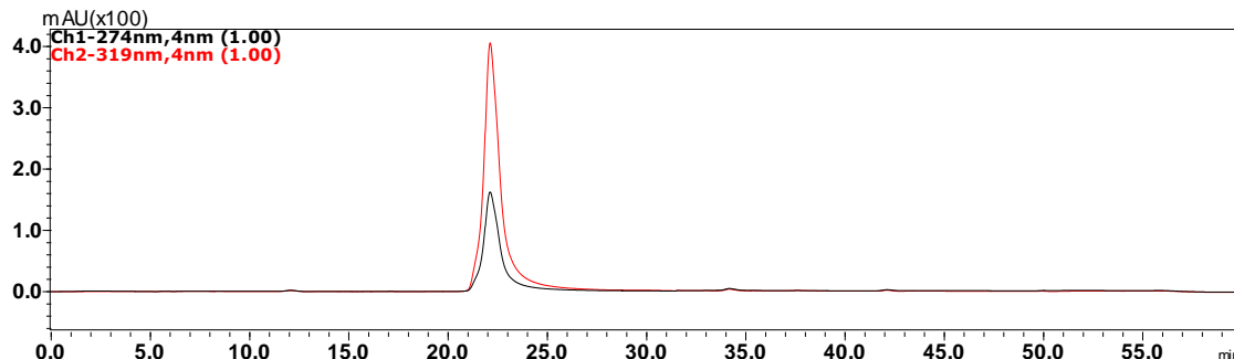
A1. 6: Exemplary RP-HPLC chromatogram of the separation of untreated chlorogenic acid detected at 274 (black) and 319 nm (red).
