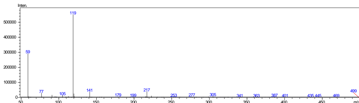
RP B (Retention time = 28.150 min)
