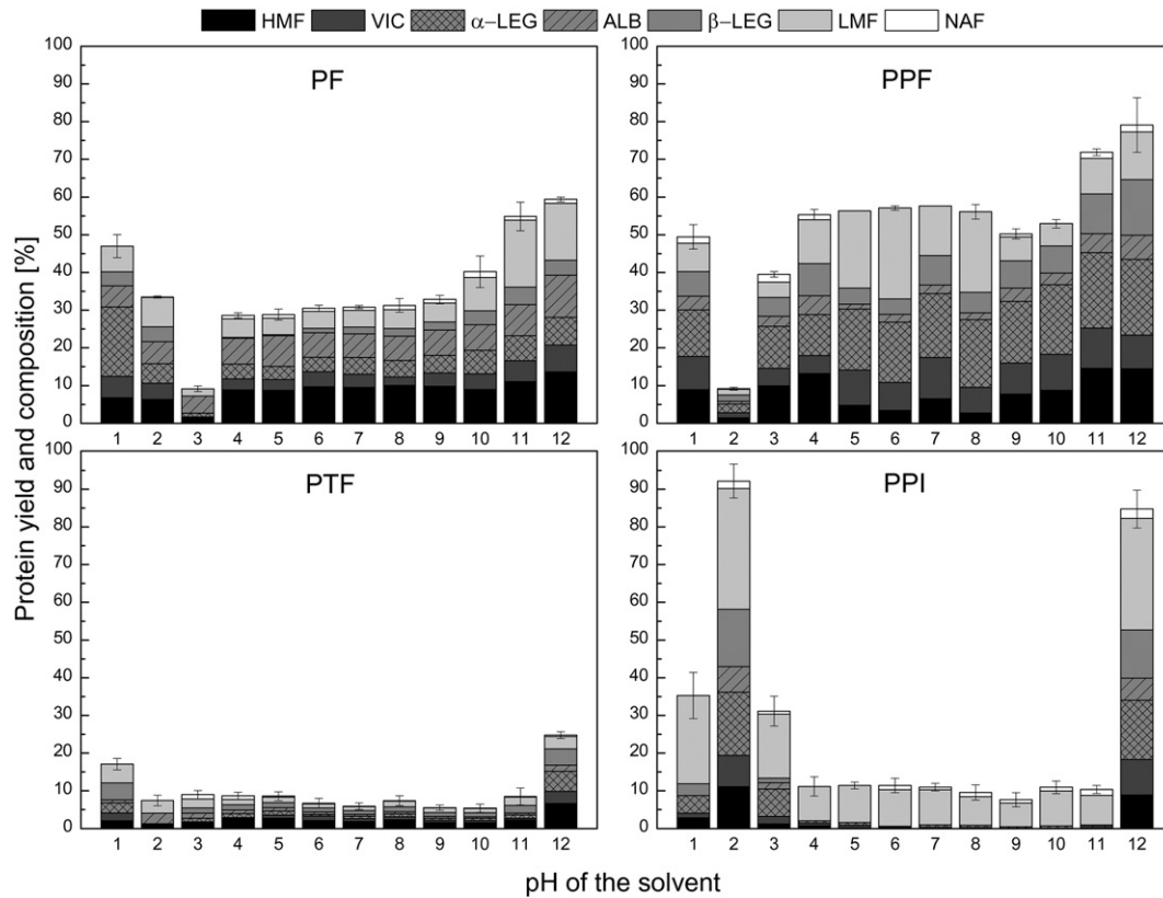
Fig. 3. Composition of the pea protein fractions (PF: pea flour, PPF: protein-rich pea flour, PTF: pea testa flour, and PPI: pea protein isolate) depending on the pH value of the extraction solution. (HMF: high molecular fraction, VIC: vicilin, \alpha -LEG: \alpha -legumin, ALB: albumin, \beta -LEG: \beta -Legumin, LMF: low molecular fraction, NAF: none allocated fraction); n = 3 .
