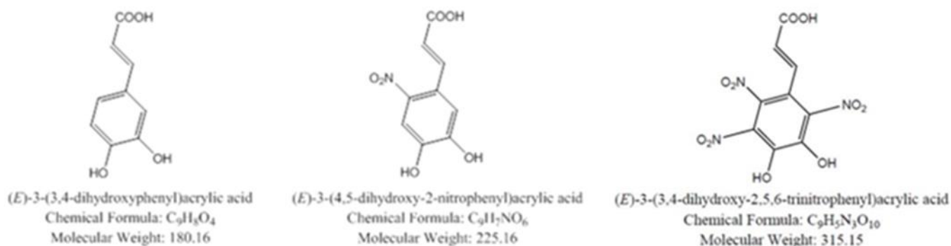
Figure 8: Proposed products of chlorogenic acid under conditions of the PPA-mediated reaction.
