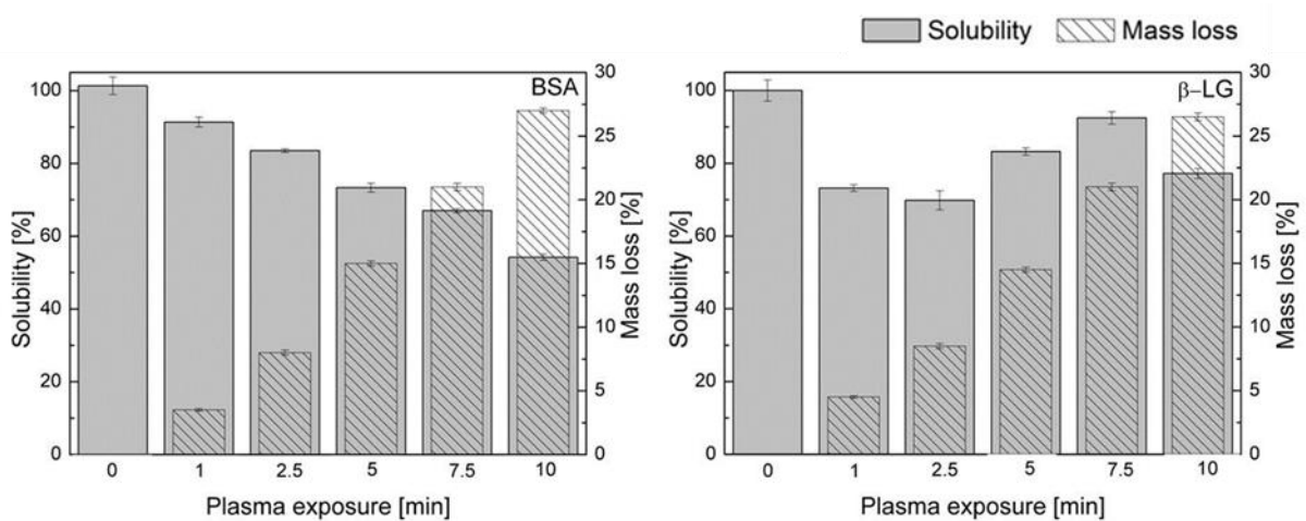
A2. 3: Plasma-induced impact on protein solubility (pH 7.0, Biuret method - grey) and mass loss (hatched) of \beta -LG and BSA solutions (Bußler, unpublished data).
