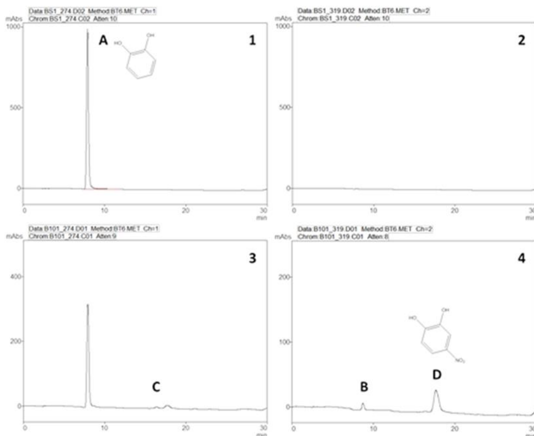
Figure 5: Exemplary RP-HPLC chromatogram of the separation of pyrocatechol detected at 274 (1) and 319 nm (2) and plasma-induced adducts RPA, RPB and RPC detected at 274 (3) and 319 nm (4) in pyrocatechol solution (10 mM) after a 10 min exposure to PPA. Code: A = Catechol; B = RP A; C = RP B; D = RP C.
