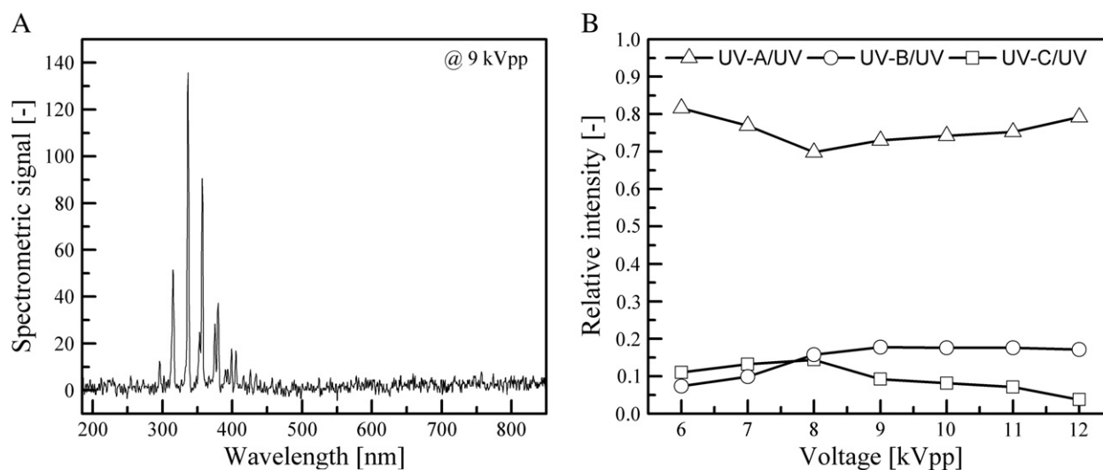
Fig. 2. (A) Optical emission spectra of the plasma generated with the SDBD device in air at an applied voltage of 9 kV pp (3.0 kHz, 20 mm distance from the plasma source). (B) Relative composition of UV-radiation (UV-A, UV-B and UV-C) at various voltages ranging from 6 to 12 kV pp (3.0 kHz, 20 mm distance from the plasma source).
