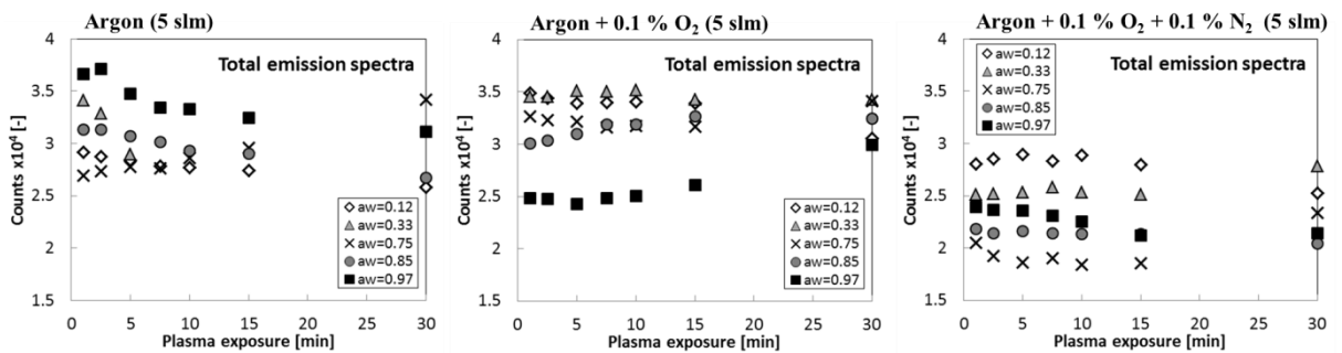
Figure 26: Area of the total emission spectra of the plasma afterglow (plasma jet kINPen©) during exposure to solid model systems with varying a_w -values under variation of the working gas measured via optical emission spectroscopy (Bußler, unpublished data).
