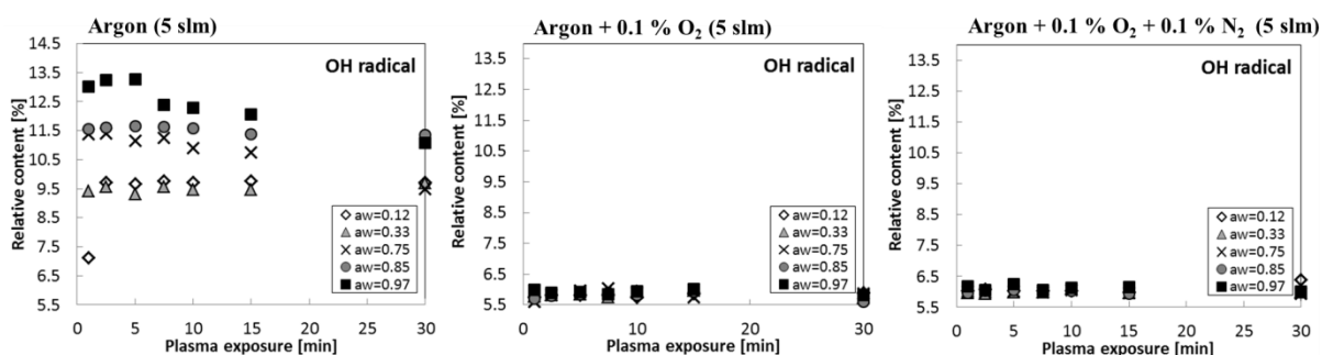
A3. 1: Relative OH content of the plasma afterglow during exposure to solid model systems with varying a_w -values under variation of the working gas measured via optical emission spectroscopy (Bußler, unpublished data).
