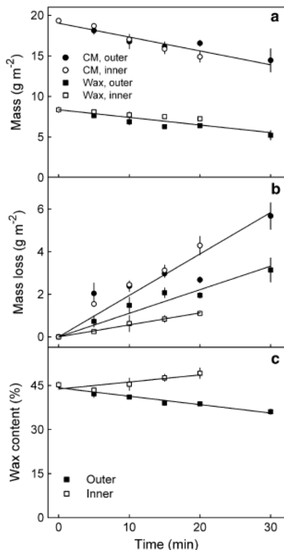
Fig. 2 Effect of the duration of cold atmospheric pressure plasma (CAPP) treatment of the morphological inner (inner) or morphological outer surfaces (outer) of cuticular membranes (CM) isolated from mature ‘Idared’ apple fruit ( Malus 9 domestica ) on the CM and wax mass per unit area (a), the loss in CM and wax mass per unit area (b), and the wax content of the CM (c). Data points represent mean \pm SE, n = 5 – 9 (treated) and 11 (untreated).
