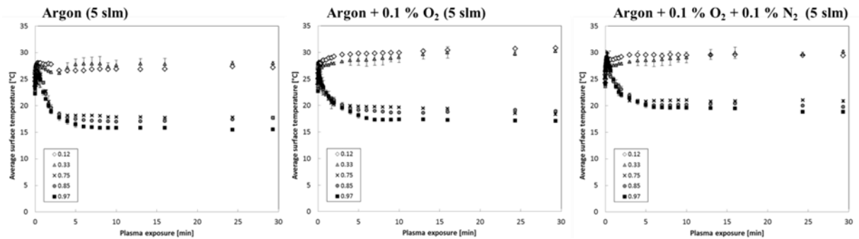
Figure 25: Time dependent average surface temperature of solid model systems with varying a_w -values exposed to direct CAPP treatment (plasma jet kINPen©) under variation of the working gas (Bußler, unpublished data).
