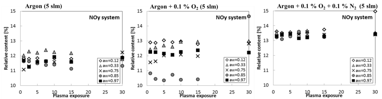
A3. 3: Relative NO_y content of the plasma afterglow during exposure to solid model systems with varying a_w -values under variation of the working gas measured via optical emission spectroscopy (Bußler, unpublished data).
