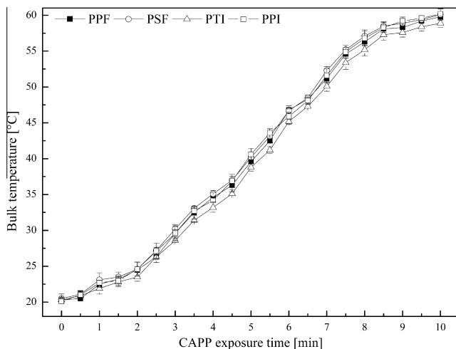
Fig. 1. Thermal bulk load of PPF, PSF, PTF and PPI during exposure to CAPP (3.0 kHz, 8.8 kVpp) for 10 min.
