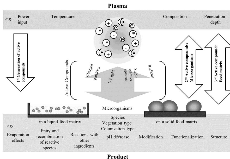
Figure 7: Product-process interactions that may take place during plasma treatment of liquid and solid food matrices.
