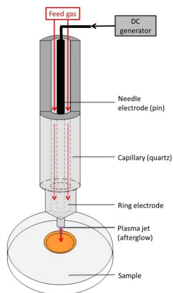
Figure 4: Schematic depiction of a plasma jet (kINPen 09, INP Greifswald) operating at atmospheric pressure conditions.
