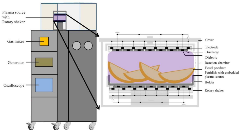
Figure 5: Schematic depiction of a DBD plasma device operating at atmospheric pressure conditions (adapted from 'LegUMAX', INP Greifswald).
