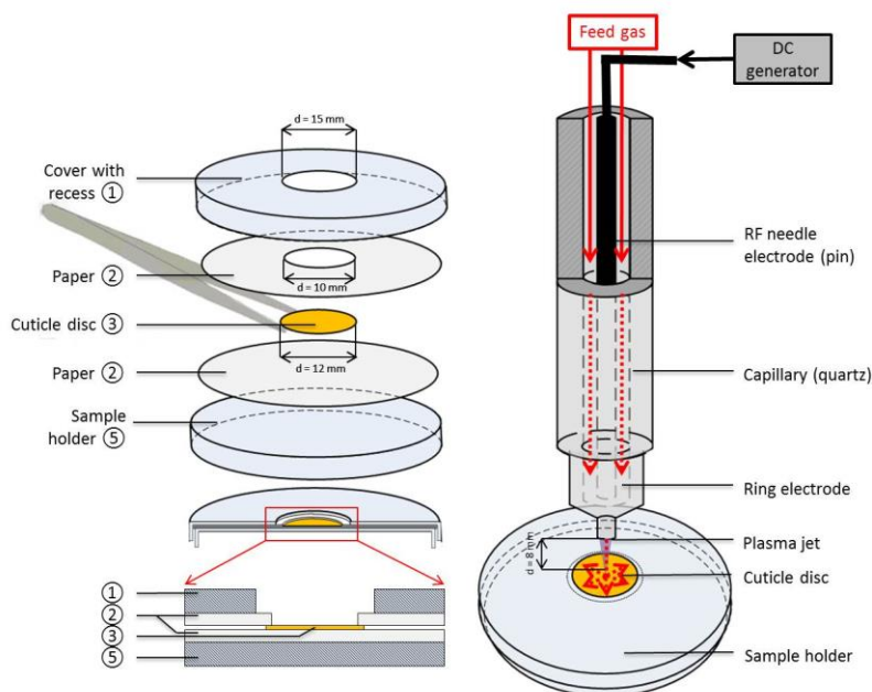
Figure 13: Design of experimental plasma-jet set-up applicable to ablate wax and cell layers from fruit cuticle surfaces in a targeted manner.
