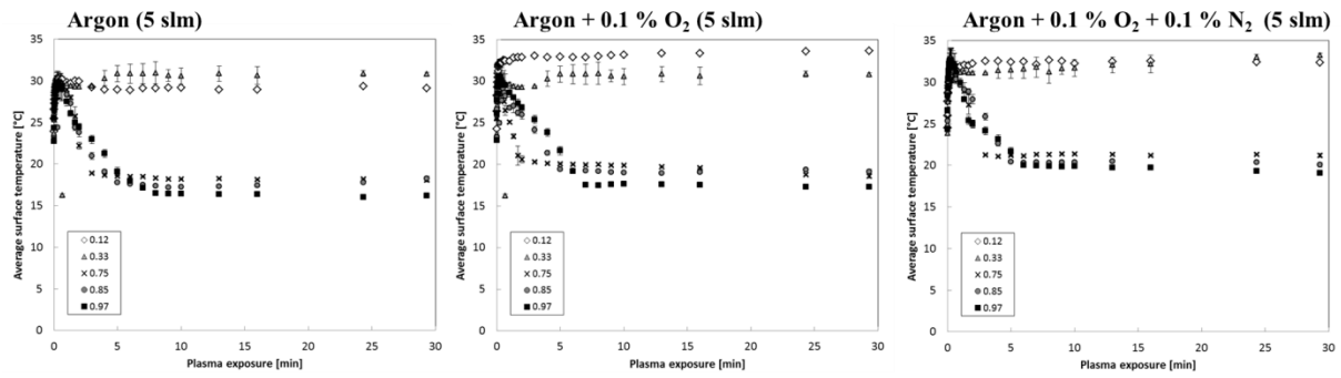
A3. 5: Time dependent average surface temperature of liquid model systems with varying a_w -values exposed to direct CAPP treatment under variation of the working gas (Bußler, unpublished data).
