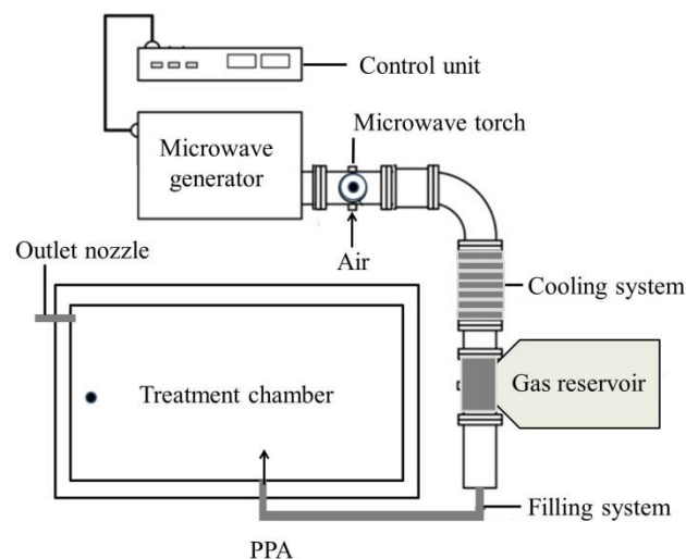
Figure 6: Schematic depiction of a microwave-driven plasma device for the generation of PPA.
