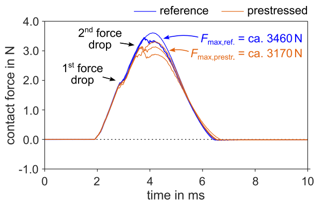
Fig. 8 Comparison of the moving average filtered curves showing the contact force response of impacted CFRP specimens for a non-prestressed reference and a prestressed compression-tension state ( -15 kN/ +15 kN)
