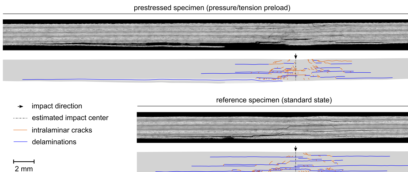
Fig. 11 Light microscopical images of the cross sections of two impacted specimen. Top: Sample of a specimen biaxially preloaded with -15\text{ kN} (axis 1) and +15\text{ kN} (axis 2). Bottom: Reference specimen without mechanical preloading
