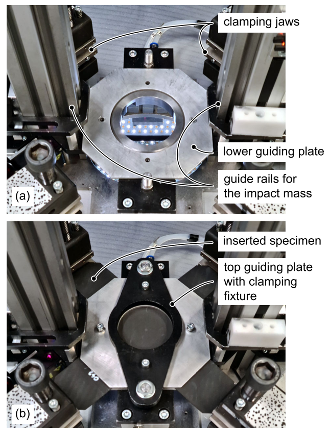
Fig. 3 Circular support before insertion of the specimen (a) and after installation (b)
