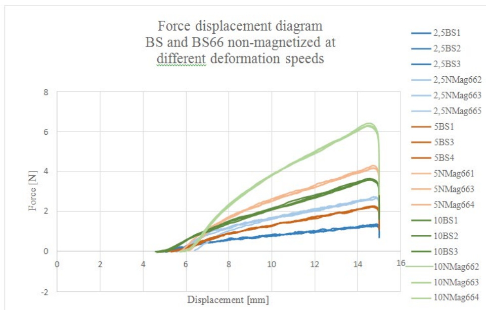
Figure 8: Graphical comparison of the force-displacement curves of pure BPA-free borosilicate and borosilicate with 66% NdPrFeB particles by weight.
