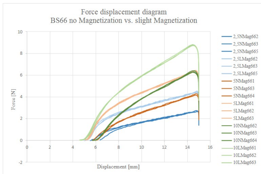
Figure 4: Influence of slight re-magnetization compared to nonre-magnetized samples in the force-displacement diagram.
