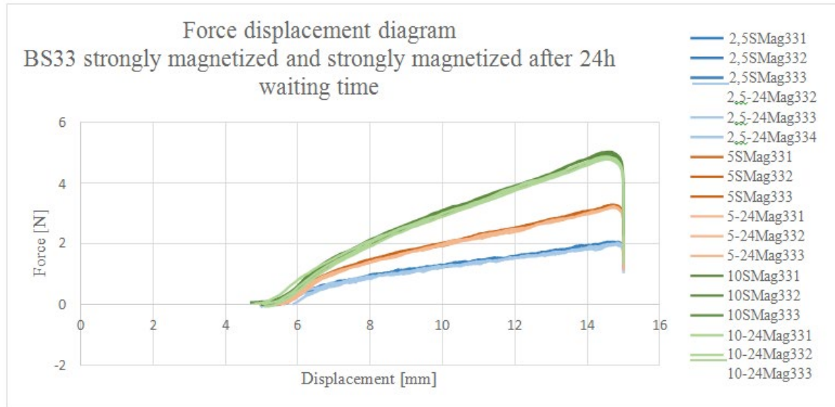
Figure 6: Graphical comparison of the force-displacement curves of the strongly remagnetized samples directly after magnetization and 24 h later in the force-displacement diagram. (33 % NdPrFeB).
