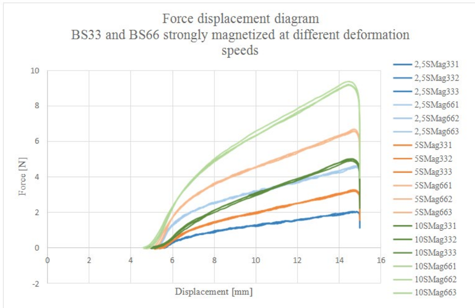
Figure 10: Graphical comparison of the force-displacement curves of borosilicate with 33% by weight NdPrFeB particles and borosilicate with 66% by weight NdPrFeB particles strongly remagnetized.
