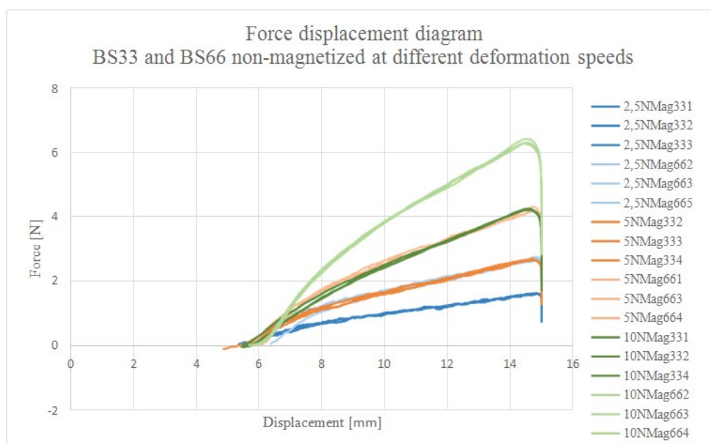
Figure 9: Graphical comparisons of the force-displacement curves of borosilicate with 33% by weight of NdPrFeB particles and borosilicate with 66% by weight of NdPrFeB particles not remagnetized.
