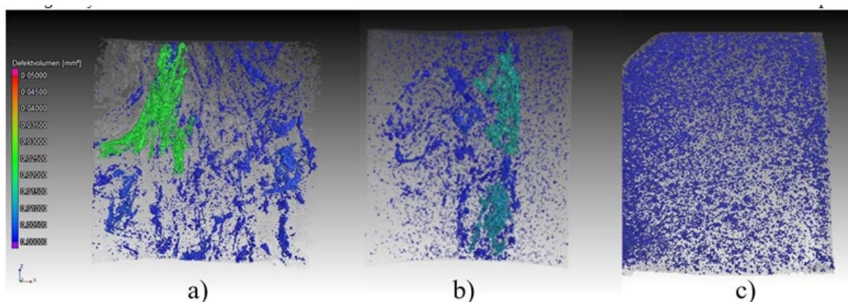
Figure 2: X-ray image of a 5% MBP sample a) after 2 passes; b) after 10 passes; c) after 20 passes.
