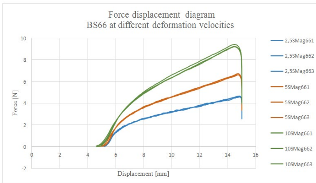
Figure 12: Graphical comparison of force-displacement curves of borosilicate with 66% wt NdFePrB particles for different velocities.
