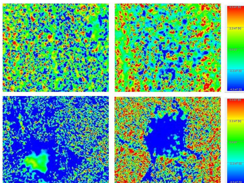
Figure 13: Image of post-magnetized samples (top) 33% wt NdPrFeB particles (bottom) 66% wt NdPrFeB particles.
