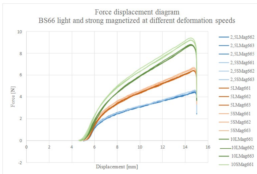
Figure 5: Graphical comparison of the force-displacement curves of the slightly magnetized to the strongly magnetized samples in the force-displacement diagram.
