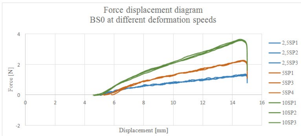
Figure 11: Graphical comparison of the force-displacement curves of borosilicate without NdPrFeB particles for different velocities.
