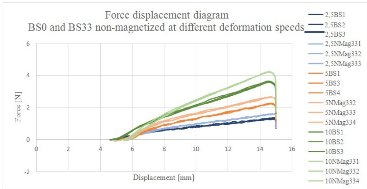
Figure 7: Graphical comparison of the force-displacement curves of pure BPA-free borosilicate and borosilicate with 33 % by weight NdPrFeB particles.
