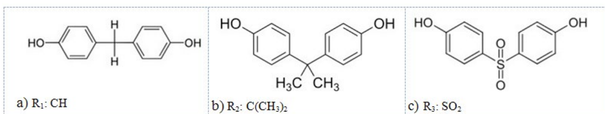
Figure 1: Bisphenol structure showing: a) Bisphenol-F (Formaldehyd), b) Bisphenol-A (Aceton), c) Bisphenol-S.
