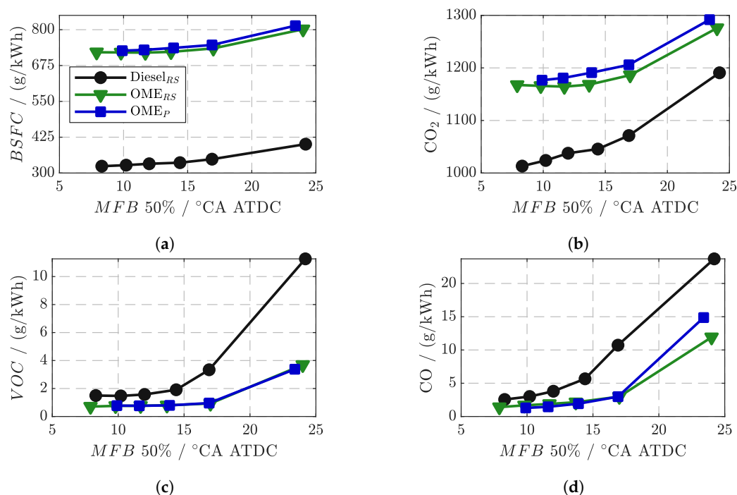
Figure 7. Brake-specific fuel consumption (a) and different specific effective emissions (b–d) for a variation of MFB 50% at OP 1 (n = 2600 1/min, BMEP = 2.2 bar) for two different nozzles in OME operation.
