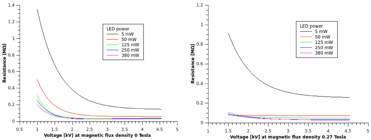
Fig. 10 Illuminated GaAs a without magnetic field, b with 0.27 T magnetic flux density
