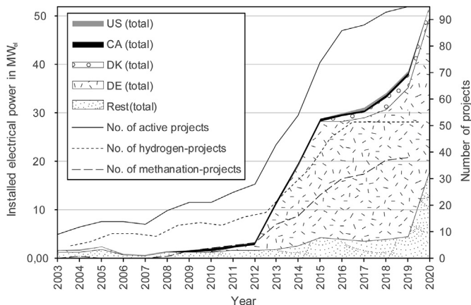
Fig. 7. Annual development of installed electrical power in PtG-projects split up in detail for the four main stakeholder countries Germany (DE), Denmark (DK), United States of America (US) and Canada (CA).
