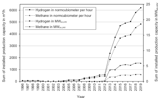
Fig. 11. Hydrogen and methane production capacity development between the years 1996 and 2019 in norm-cubic meter per hour and related to the lower heating value LHV ( LHV_{H_2} = 2.995 \text{ kWh/m}^3 , LHV_{CH_4} = 9.986 \text{ kWh/m}^3 ).
