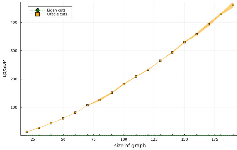
Fig. 12 Quotients for the Lovász theta number \frac{z_{\mathcal{L}}}{z_{sdp}} and \frac{z_n}{z_{sdp}} as n grows for random d -regular graphs with d = \frac{n}{10}
