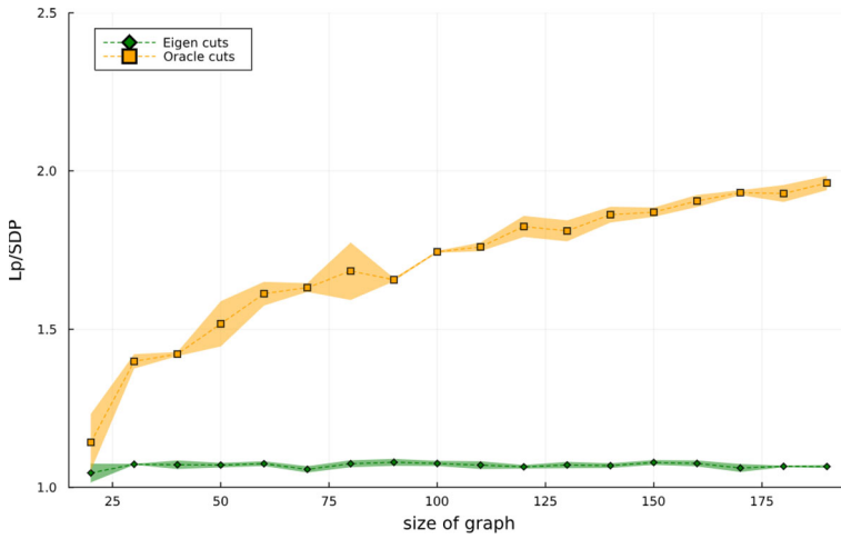
Fig. 5 Ratio of \frac{z_{\mathcal{L}}}{z_{sdp}} (Eigen cuts) and \frac{z_n}{z_{sdp}} (Oracle cuts) for instances of max cut where the graph is a random d -regular graph, with d = \sqrt{n} , as n grows
