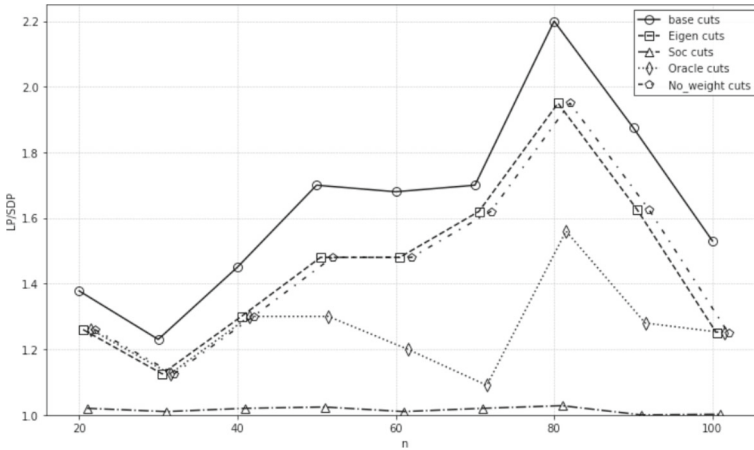
Fig. 25 Quality of the ratios \frac{z_{LP}}{z_{SDP}} (eigen cuts), \frac{z'_{LP}}{z_{SDP}} (no_weight cuts), \frac{z_n}{z_{SDP}} (oracle cuts), \frac{z_0}{z_{SDP}} (base cuts), and \frac{z_{soc}}{z_{SDP}} for instances of the quadratic knapsack problem with density \Delta = 0.95
