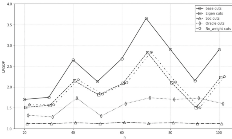
Fig. 22 Quality of the ratios \frac{z_{\mathcal{J}}}{z_{sdp}} (eigen cuts), \frac{z'_{\mathcal{J}}}{z_{sdp}} (no_weight cuts), \frac{z_n}{z_{sdp}} (oracle cuts), \frac{z_0}{z_{sdp}} (base cuts), and \frac{z_{soc}}{z_{sdp}} for instances of the quadratic knapsack problem with density \Delta = 0.25
