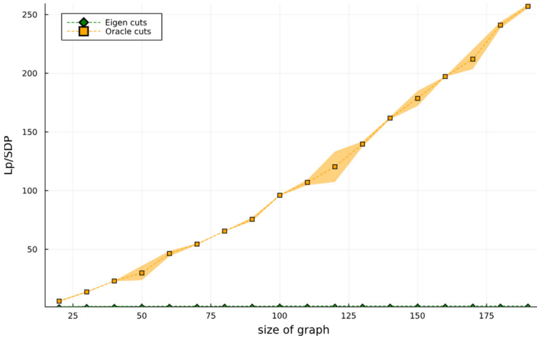
Fig. 7 Quotients for the Lovász theta number \frac{\chi(G)}{z_{sdp}} (Eigen cuts) and \frac{z_{\mathcal{F}}}{z_{sdp}} (Oracle cuts) as n grows for Erdős-Rényi random graphs with p = 0.5
