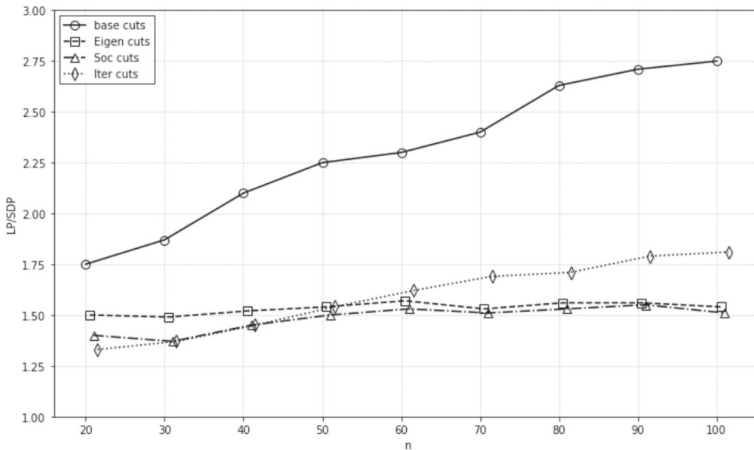
Fig. 16 Quality of the ratios \frac{z_{\mathcal{L}}}{z_{sdp}} (eigen cuts), \frac{z_n}{z_{sdp}} (oracle cuts), \frac{z_0}{z_{sdp}} (base cuts), and \frac{z_{soc}}{z_{sdp}} for random QCQP instances with r = n , and q = \frac{n}{10}
