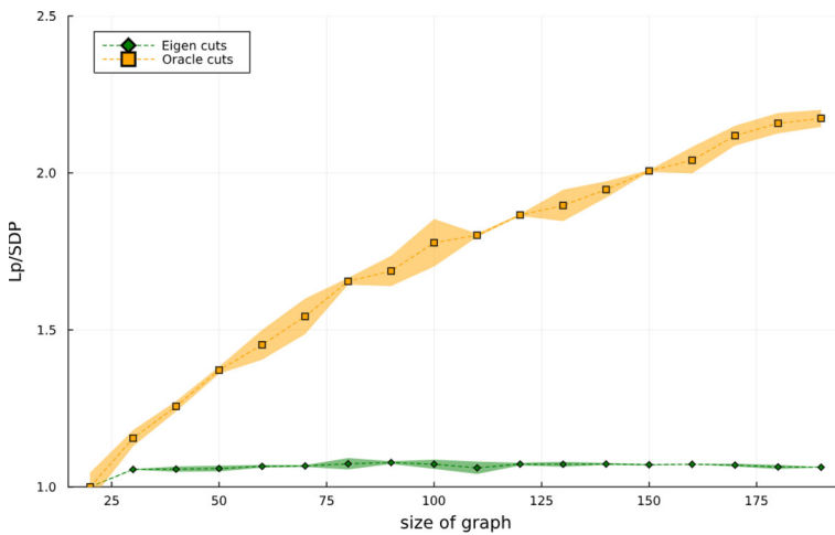
Fig. 6 Ratio of \frac{z_{\mathcal{L}}}{z_{sdp}} (Eigen cuts) and \frac{z_n}{z_{sdp}} (Oracle cuts) for instances of max cut where the graph is a random d -regular graph, with d = \frac{n}{10} , as n grows
