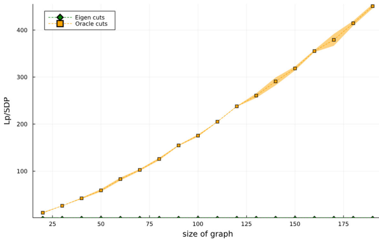
Fig. 11 Quotients for the Lovász theta number \frac{\theta(G)}{z_{sdp}} and \frac{z_n}{z_{sdp}} as n grows for random d -regular graphs with d = \sqrt{n}
