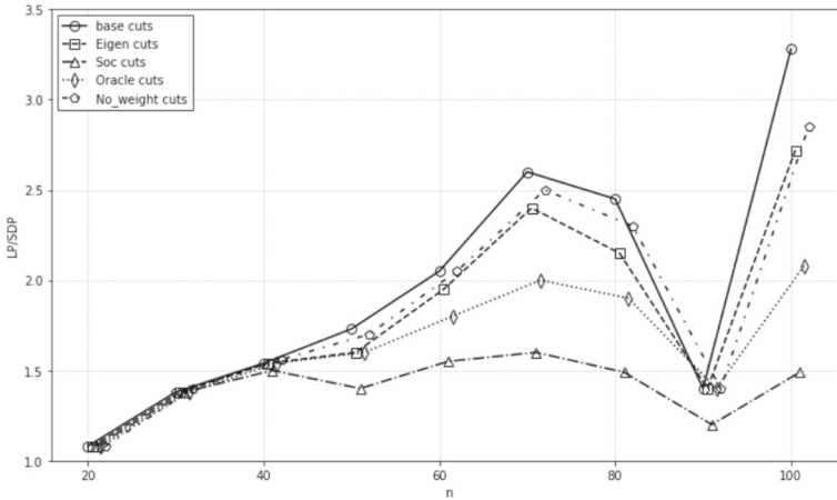
Fig. 21 Quality of the ratios \frac{z_{\mathcal{J}}}{z_{sdp}} (eigen cuts), \frac{z'_{\mathcal{J}}}{z_{sdp}} (no_weight cuts), \frac{z_n}{z_{sdp}} (oracle cuts), \frac{z_0}{z_{sdp}} (base cuts), and \frac{z_{soc}}{z_{sdp}} for instances of the quadratic knapsack problem with density \Delta = 0.05
