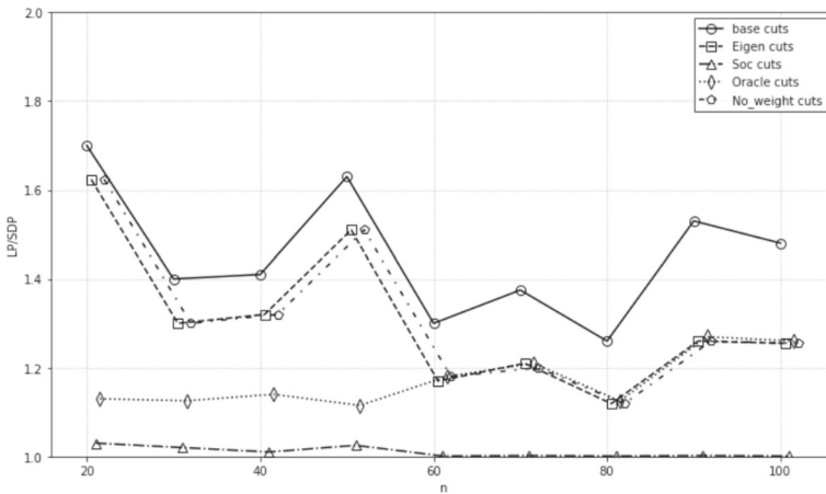
Fig. 26 Quality of the ratios \frac{z_{LP}}{z_{SDP}} (eigen cuts), \frac{z'_{LP}}{z_{SDP}} (no_weight cuts), \frac{z_n}{z_{SDP}} (oracle cuts), \frac{z_0}{z_{SDP}} (base cuts), and \frac{z_{soc}}{z_{SDP}} for instances of the quadratic knapsack problem with density \Delta = 1
