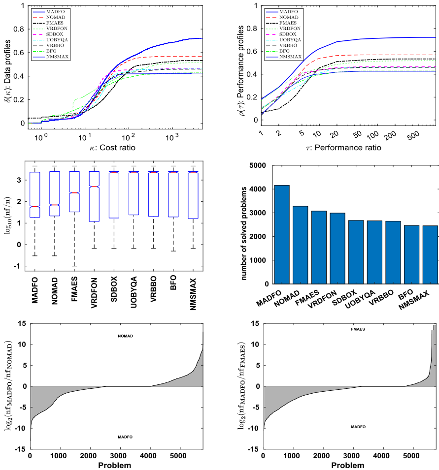
Fig. 10 Data and performance profiles (first row), box plots and bar graphs (second row), and Morales profiles (third row) for noisy problems with the quadratic f . Other details as Fig. 7
