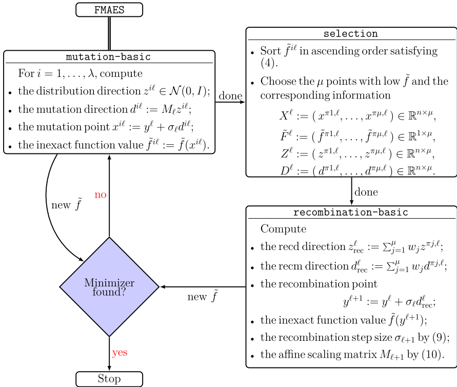
Fig. 1 Pseudocode for FMAES. X_i denotes the i th column of the matrix X
