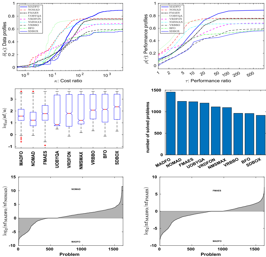
Fig. 8 Data and performance profiles (first row), box plots and bar graphs (second row), and Morales profiles (third row) for noisy problems with the quadratic f . Other details as Fig. 7
