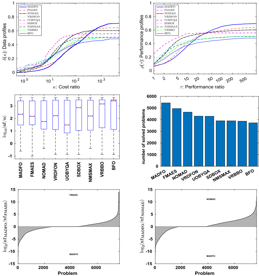
Fig. 9 Data and performance profiles (first row), box plots and bar graphs (second row), and Morales profiles (third row) for noisy problems with the quadratic f . Other details as Fig. 7
