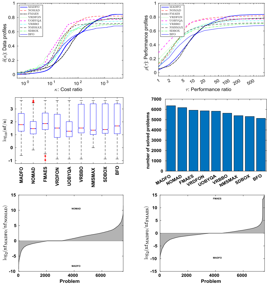
Fig. 11 Data and performance profiles (first row), box plots and bar graphs (second row), and Morales profiles (third row) for noisy problems with all types of f and the 4 small noise levels \omega = 10^k for k = -5, -4, -3, -2 . Other details as Fig. 7
