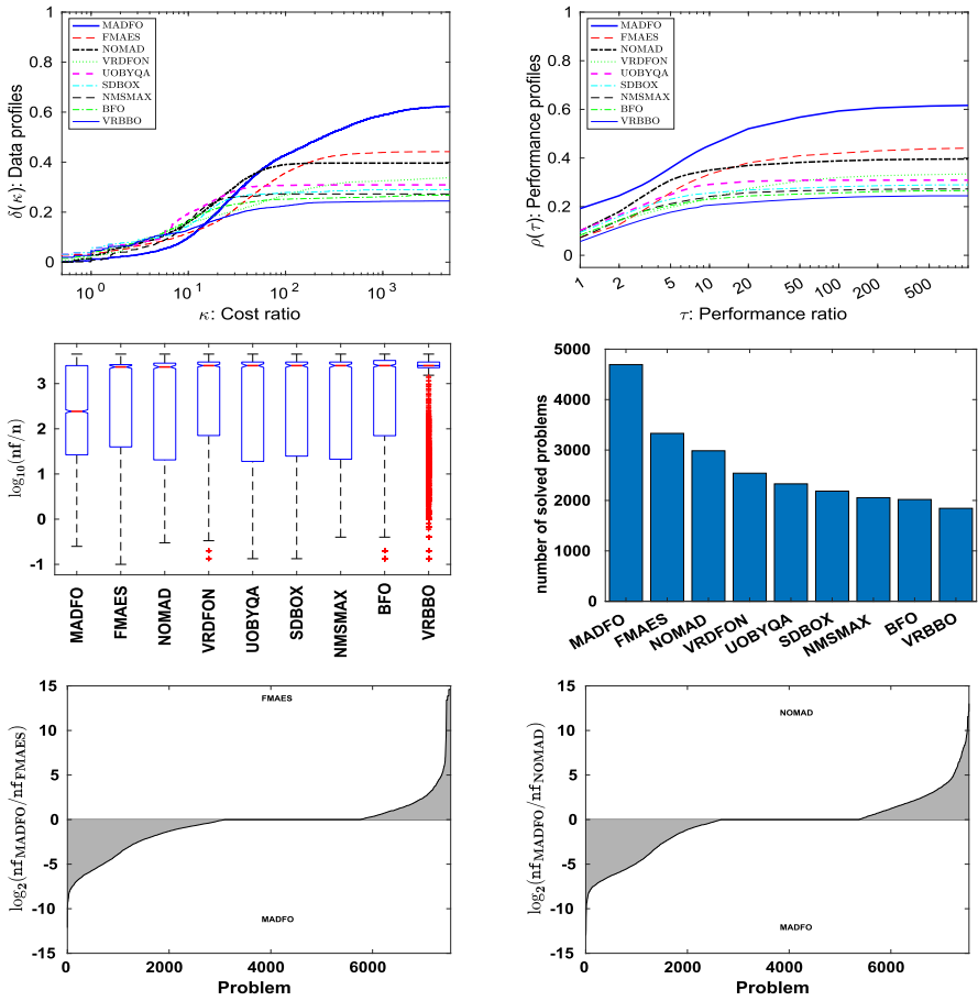
Fig. 12 Data and performance profiles (first row), box plots and bar graphs (second row), and Morales profiles (third row) for noisy problems with all types of f and the 4 large noise levels \omega = 10^k for k = -1, 0, 1, 2 . Other details as Fig. 7
