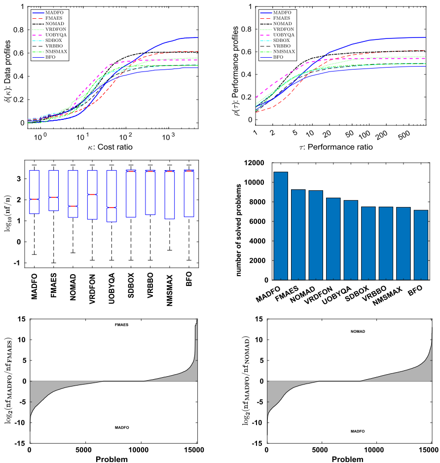
Fig. 7 Data and performance profiles (first row), box plots and bar graphs (second row), and Morales profiles (third row) for noisy problems with all types of f and small dimensions 1 < n \leq 20 , generated by the absolute/relative uniform and Gaussian noises, the three target accuracies \varepsilon \in \{10^{-4}, 10^{-3}, 10^{-2}\} , and the noise levels \omega = 10^k for k = -5, -4, \dots, 2 . Problems solved by no solver are ignored. All 9 compared solvers used the budgets secmax = 360 and nfmax = 2000n + 5000
