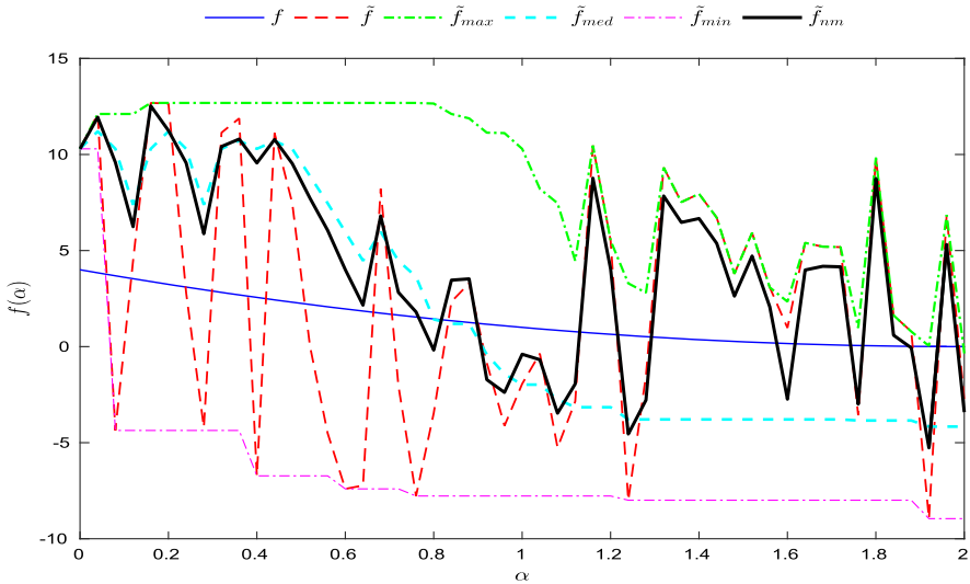
Fig. 5 A plot of the exact function values f , the noisy function values \tilde{f} , the values \tilde{f}_{max} , \tilde{f}_{min} , and \tilde{f}_{med} from (14), and the new noisy non-monotone term values \tilde{f}_{nm} of the one-dimensional objective function f(\alpha) = (\alpha - 2)^2 for \alpha \in [0, 2] . Absolute uniform noise with noise level 1 was used
