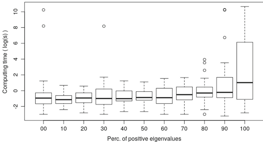
Fig. 2 Distribution of computing time (log scale) of (K_{\delta^*, \rho^*}\text{-QP-}kn) on CD instances
