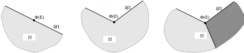
Figure 3: Cut through \Pi_\bullet perpendicular to \Phi(E) for a monomaterial segment, a monomaterial edge and a bimaterial edge, respectively
