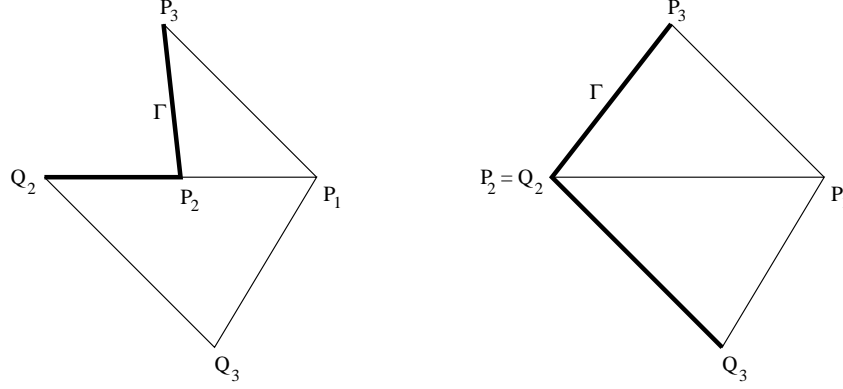
Figure 2: The basis of the prism \mathcal{P} and of the Neumann boundary part \Gamma in the two cases P_2 \neq Q_2 and P_2 = Q_2
