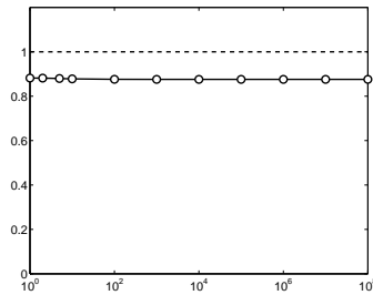
Fig. 5 Effectivity ratios over inverse temperature.
