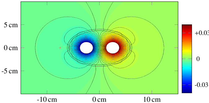
Figure 2: Flux lines and magnitude of magnetic field for an elliptic thin sheet (dashed lines) computed by the integral equation (16) and ITC-1-0. The red cross indicates the point (-7.5 \text{ cm}, 0 \text{ cm}) where we study the shielding efficiency.
