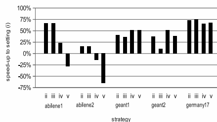
(c) speed-up compared to CPLEX (strategy (i))
