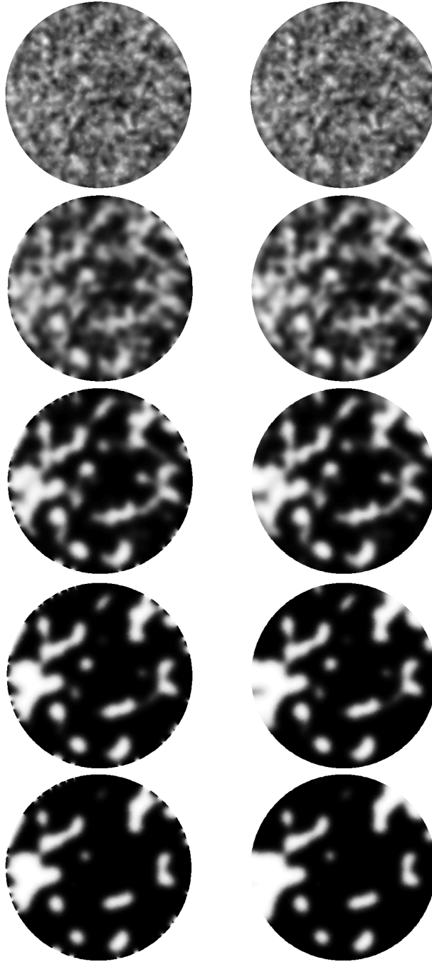
Figure 2: Numerical examples for Allen–Cahn equation ( AC_{\text{bulk}} ) in circular domain with dynamic boundary condition (12) (left) and homogeneous Neumann boundary condition (right) for double well potential W_b(u) = W_s(u) = (1 - u^2)^2 and A_b = 1000 \cdot A_s and \tau_b = \tau_s .
