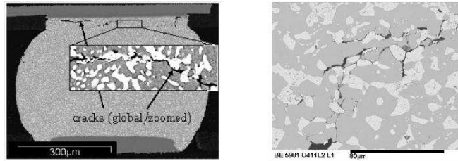
Figure 2: Initiation and propagation of cracks along the phase boundary [FBFD06].
