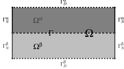
FIG. 1.1. Heterostructure \Omega with interface \Gamma .
