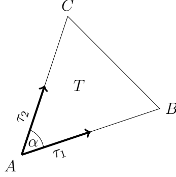
FIGURE 3.1. Geometry in Theorem 3.1.
