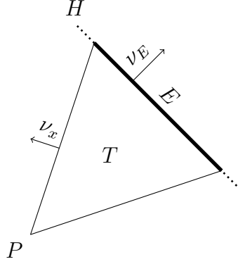
FIGURE 2.1. Geometry of the triangle T from Lemma 2.1 and Lemma 2.3.
