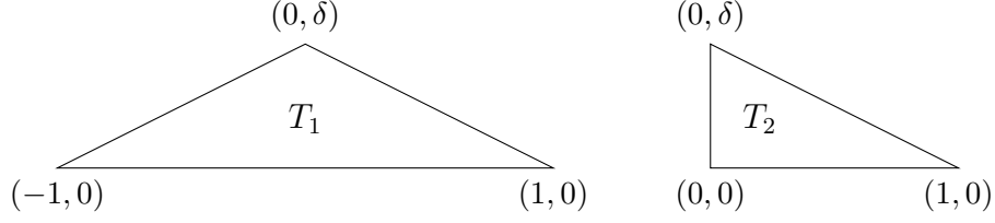
FIGURE 3.2. The triangles T_1 and T_2 from Example 3.2.
