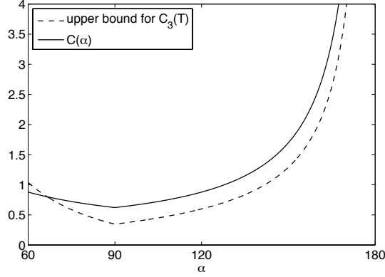
FIGURE 3.3. Comparison of the constant C(\alpha) and the upper bound (3.1) for C_3(T) .
