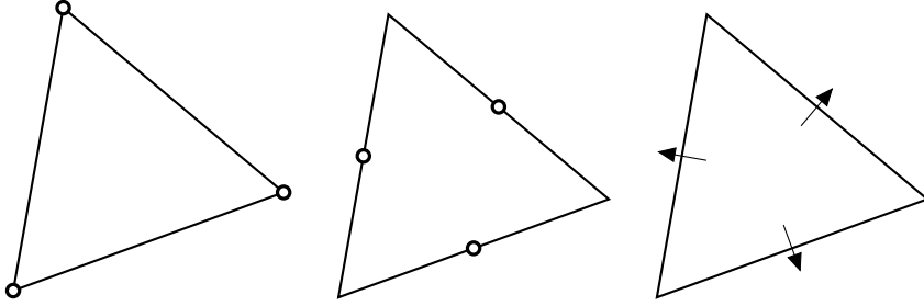
FIGURE 1.1. Courant, Crouzeix-Raviart, and Raviart-Thomas FE.
