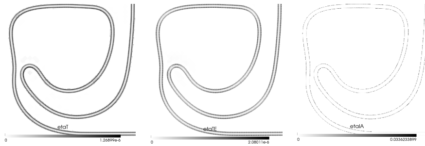
Figure 7.5: Error indicators \eta_T (left), \eta_{TE} (middle) and \eta_{IA} (right) for adaptation at time t = 45000\tau .
