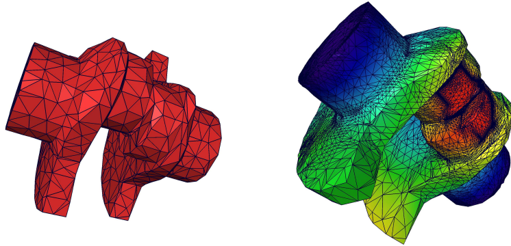
Figure 8: Crank shaft: Coarse grid (left) and adaptively refined grid (right).
