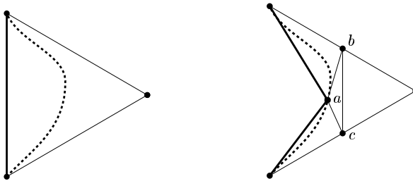
Figure 12: Refinement at a concave surface (dotted) leads to a badly shaped element (a, b, c) . If the surface was even more concave, a would pass beyond b and c , leading to an element with negative volume.
