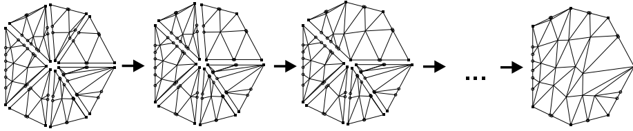
Figure 3: The flattened star of a vertex is merged into a single polygon.
