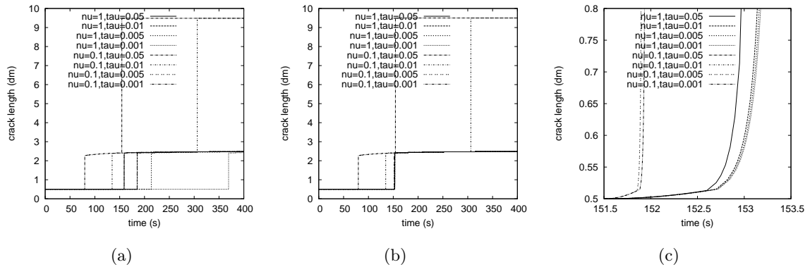
Figure 8: Approximation of the BV-solution: (a) two fixed viscosity parameters \nu_N , time step \tau_N \rightarrow 0 (Algorithm I), (b) two fixed viscosity parameters \nu_N , time step \tau_N \rightarrow 0 (Algorithm II), (c) zoom at the jump (Algorithm II).
