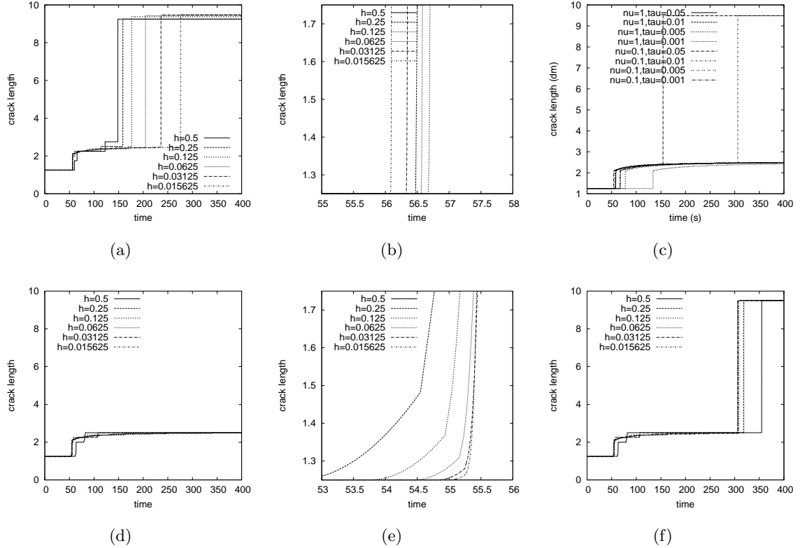
Figure 9: Approximation of the BV-solution for initial crack \mathfrak{s}_0 = 1.25 : (a) \sigma_N = h_N , \nu_N = 0.1h_N^{0.5} , \tau_N = 0.1h_N (Algorithm I), (b) zoom at the jump (Algorithm I), (c) fixed \nu_N, \tau_N \rightarrow 0 (Algorithm I), (d) \nu_N = h_N^{0.5} , \tau_N = 0.1h_N (Algorithm II), (e) zoom at the jump (Algorithm II), (f) \nu_N = \tau_N = h_N (Algorithm II).
