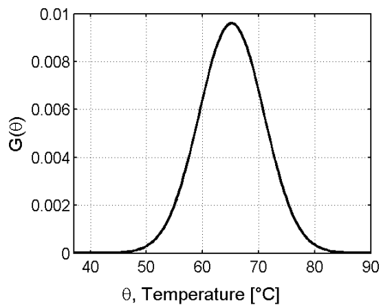
Figure 3: Function G(\theta) .
