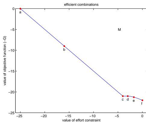
Figure 7: development of gain-optimal combinations
