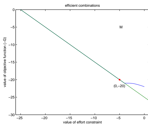
Figure 8: separation of (0, 20) by a linear functional
