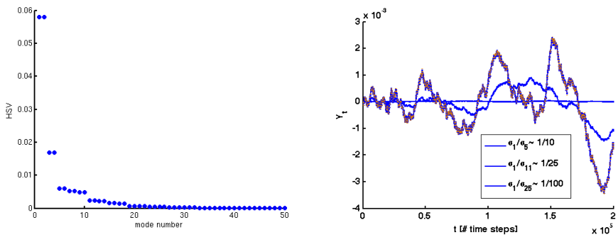
Figure 1. Left panel: The first 50 Hankel singular values of the ISS model. Right panel: Comparison between typical realizations of the third component of Y_t of the full system (dashed orange curve) and reduced systems of degrees d \in \{4, 10, 24\} ; for d = 24 the two full dynamics and the approximant are virtually indistinguishable.
