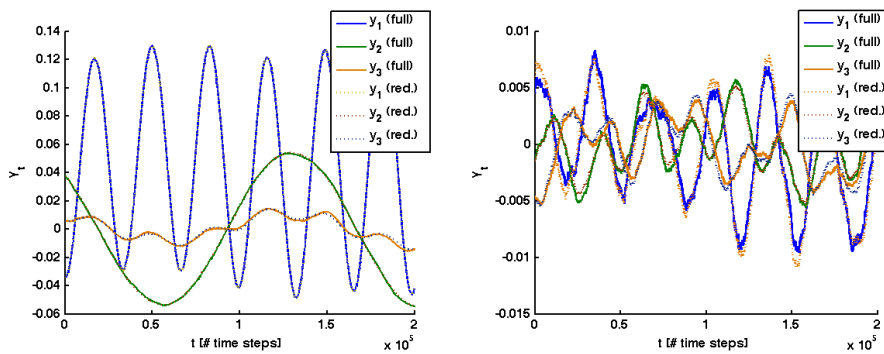
Figure 2. Left panel: Output Y_t of the full, 270-dimensional system and its 10-dimensional approximat (dashed curves) for random initial conditions restricted to the invariant subspace. Right panel: The same for Gaussian random initial conditions and an approximat of degree d = 24 .
