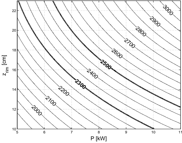
Figure 5: Illustration of state constraints (2.5) restricting the admissible (P, z_{\text{rim}}) -domain: Contour plots of \max_A \left( \frac{\partial T}{\partial z} \right) (T) , \max_{\Omega}(T) in Row (1); \min_{\Gamma}(T) , \max_{\Gamma}(T) in Row (3); \mathcal{F}_{r,2}(T) in Row (2); T = T(f, P, z_{\text{rim}}) , f = 10 \text{ kHz} , being the solution of the heat transfer problem. Values of used constraints are emphasized (cf. (4.2)).
